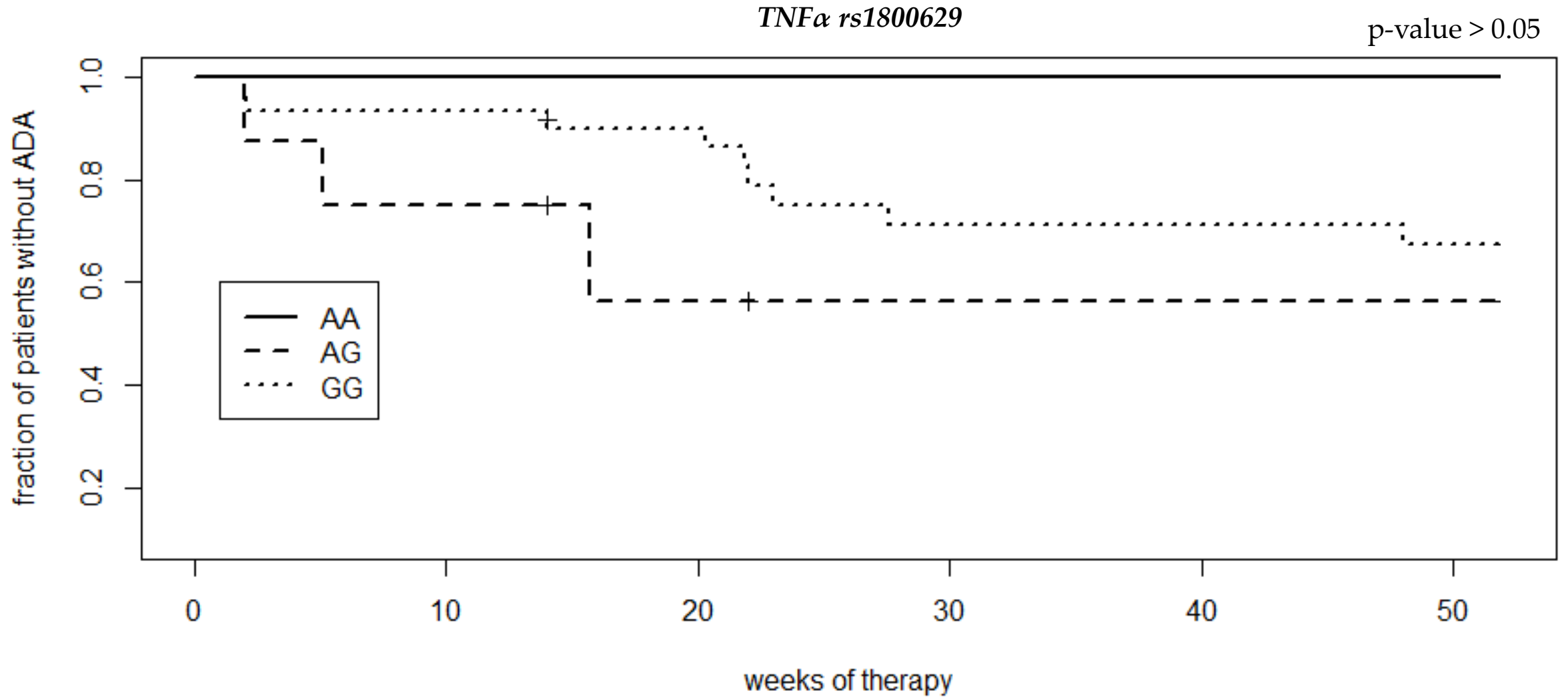
Supplementary Figure S1. Survival curves of infliximab anti-drug antibody (ADA) production according to TNF \alpha rs1800629 genotype from a Cox proportional hazard model. Dash indicates patients that have interrupted the follow up before weeks 52.
