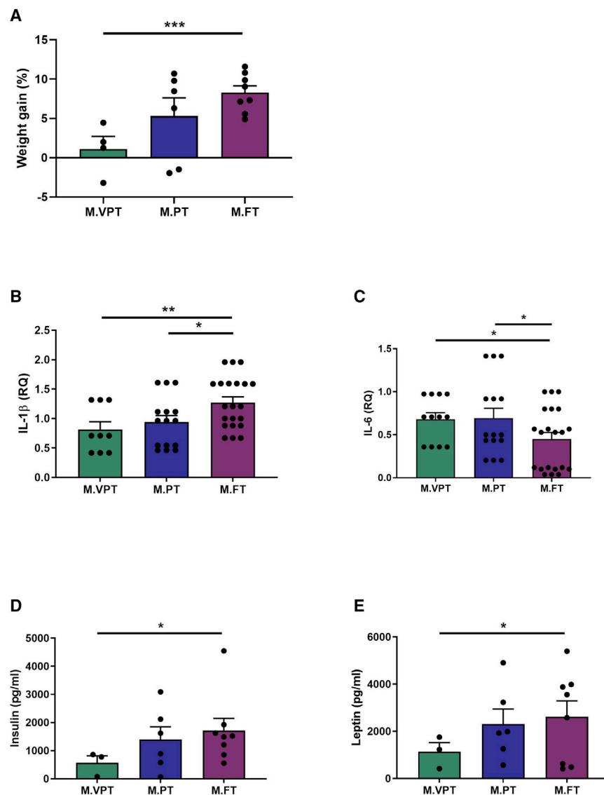
Figure 2. The effect of FMT using meconium on growth, metabolic hormones, and inflammatory cytokines in germ-free mice
