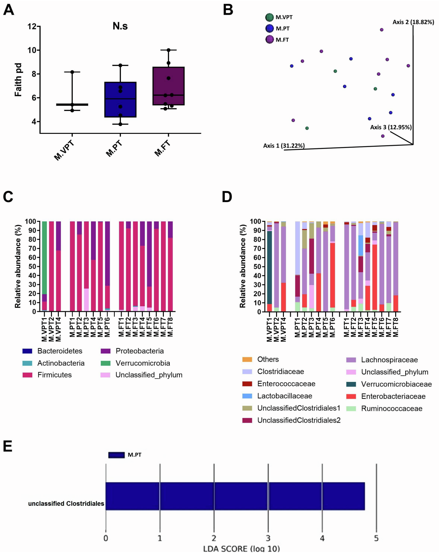
Supplemental Figure 2: Mouse microbiota composition 35 days after fecal microbiota transplant using meconium from very preterm (VPT), moderately preterm (PT) or term (FT) neonates. Related to Figure 2. (A) Gut microbial diversity was analyzed among the M.VPT (mouse, VPT), M.PT (mouse, PT) and M.FT (mouse, FT) transplanted mice 35 days after transfer by Faith's phylogenetic diversity index, compared with t-tests. Data are mean \pm SEM. NS: not significant. (B) PCoA of unweighted UniFrac distances, compared with PERMANOVA (NS). (C) Taxonomic summary at the phylum level. (D) Taxonomic summary at the family level. (E) LEfSe analysis of bacteria which are overrepresented in mice receiving FMT from PT infants.
