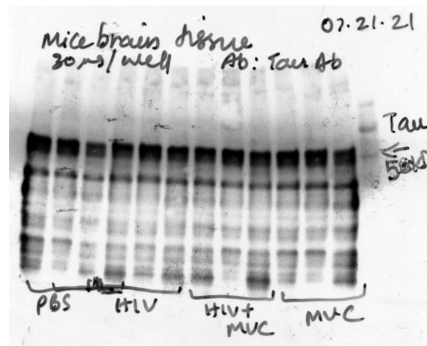
Tau
