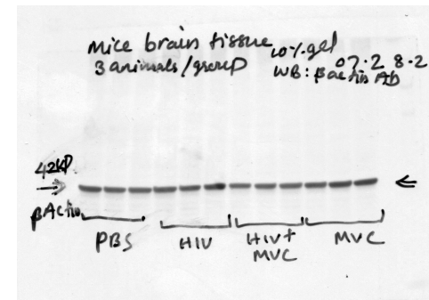
β-Actin
