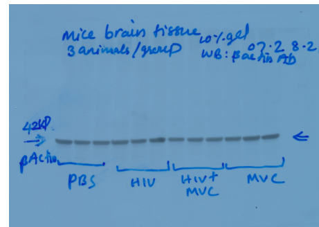
β-Actin
