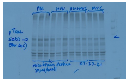
pTau (Thr205)
