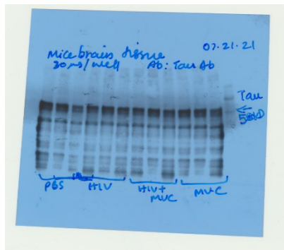
Tau
