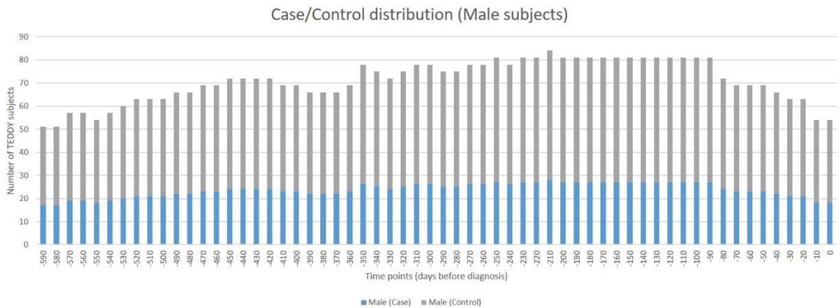
Supplementary Figure 3: T1D case control distribution at each time-point. T1D cases were grouped based on their offset in days to T1D diagnosis. In steps of 10 days, gene expression data (sample) collected from each individual closest to a particular time point was identified. For each T1D sample, at each time point, two control samples were identified that was matched on age and gender. The top panel shows sample distribution at each time point for samples collected from female study subjects and the lower panel shows sample distribution for male study subjects. In both panels, T1D case samples are marked with blue and control samples are marked with grey.
