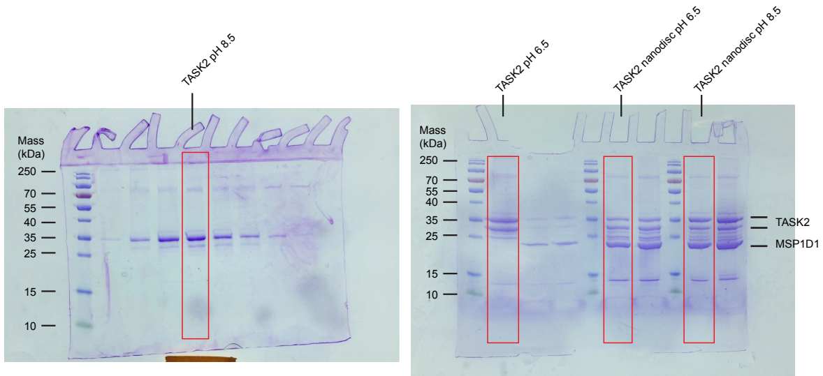
Supplementary Figure 3 | SDS-PAGE gels of purified and reconstituted TASK2. Uncropped original gel images with regions shown in Extended Data Fig. 1 outlined in red. Molecular weight of bands in marker lane is indicated.
