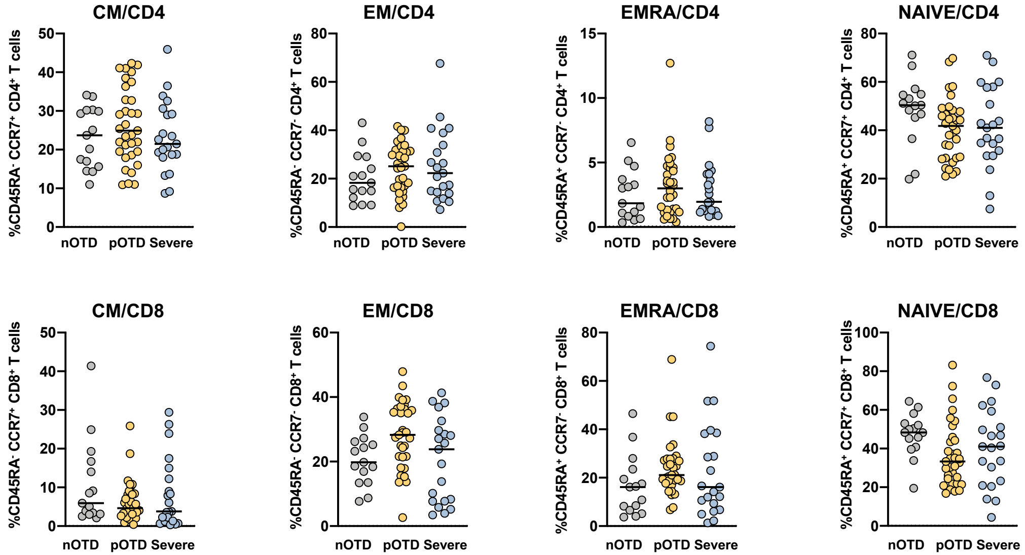
Suppl. Fig. 6 Percentage of T-cell subsets central memory (CM), effector memory (EM), effector memory CD45RA+ (EMRA) and naïve calculated out of total CD4+ (upper panel) or total CD8+ T cells (bottom panel) are shown.
