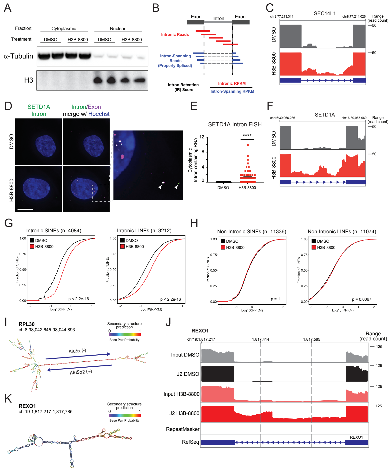
Figure S4. Intron-Retained RNAs Accumulate in the Cytoplasm and Form dsRNA, Related to Figure 4
