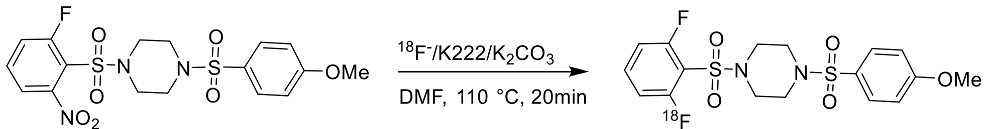
Supplemental Fig. 1. Radiosynthesis of [^{18}\text{F}] DASA-23
