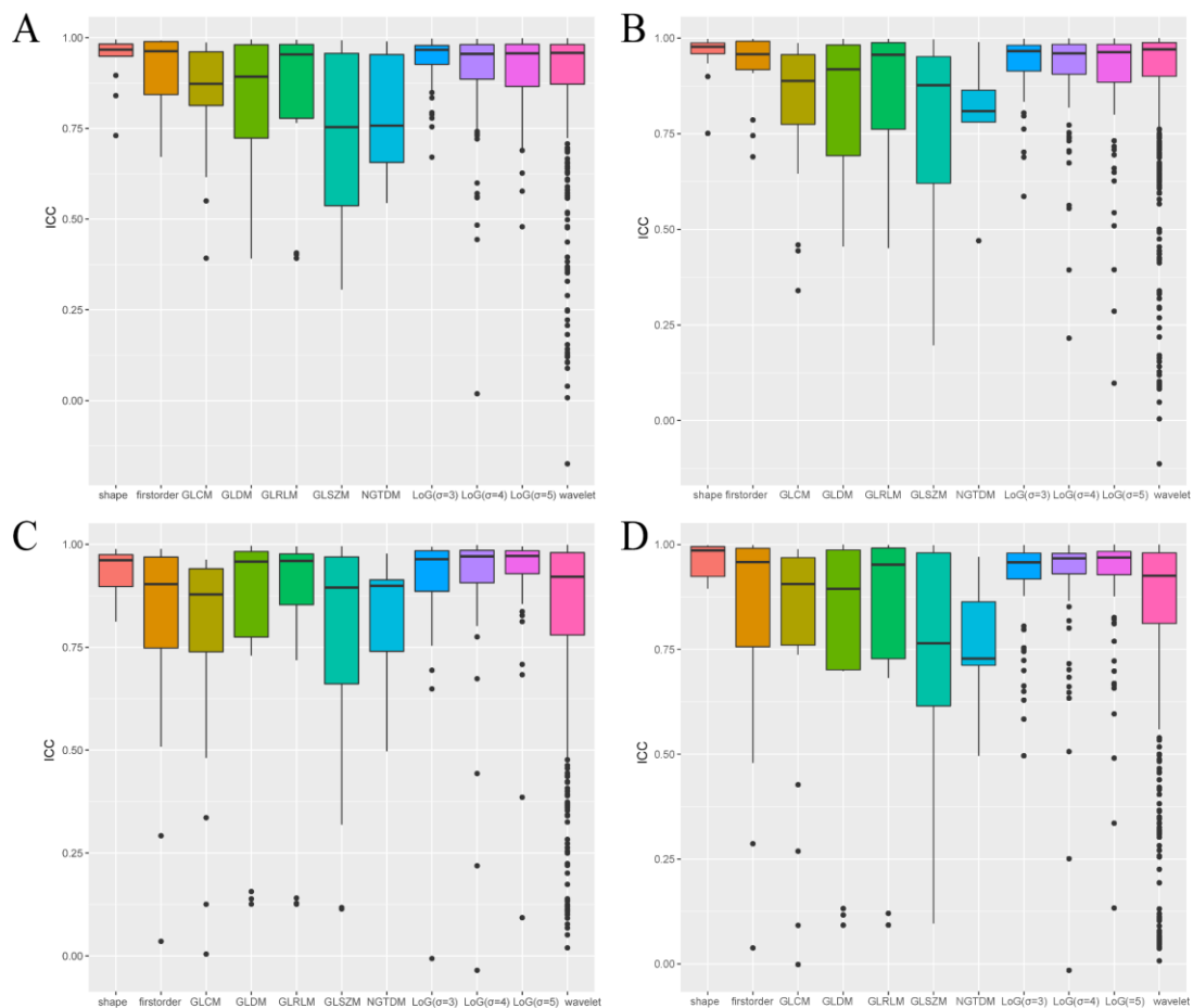
Supplementary Figure.1. Boxplot diagrams of the inter- and intra- class correlation coefficients (ICCs) for radiomic features on the CT dataset
