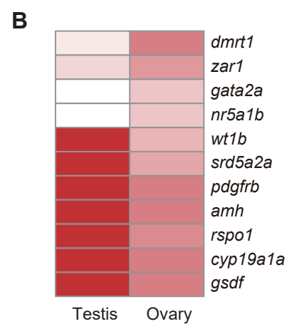
DNA methylation at promoters
