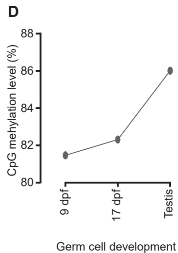
DNA methylation at promoters
