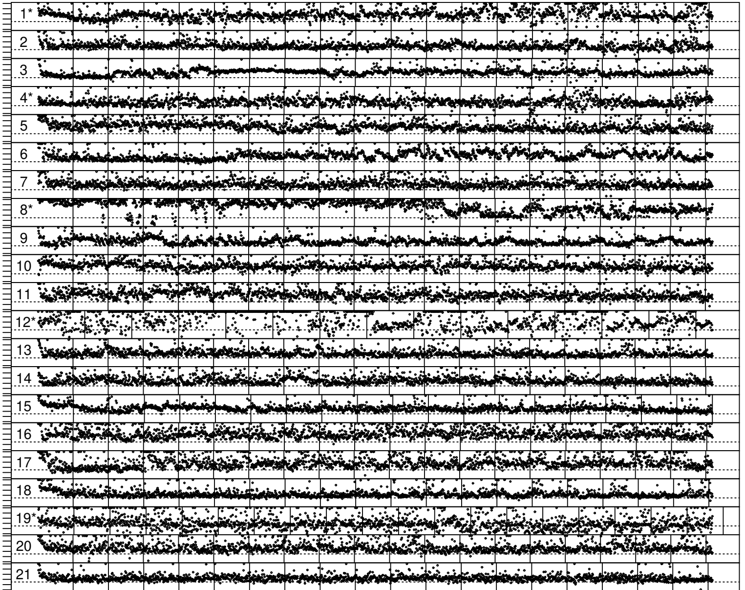
A time series plot of all RTs for all subjects for the Y25 task in Ratcliff & McKoon (2018)
