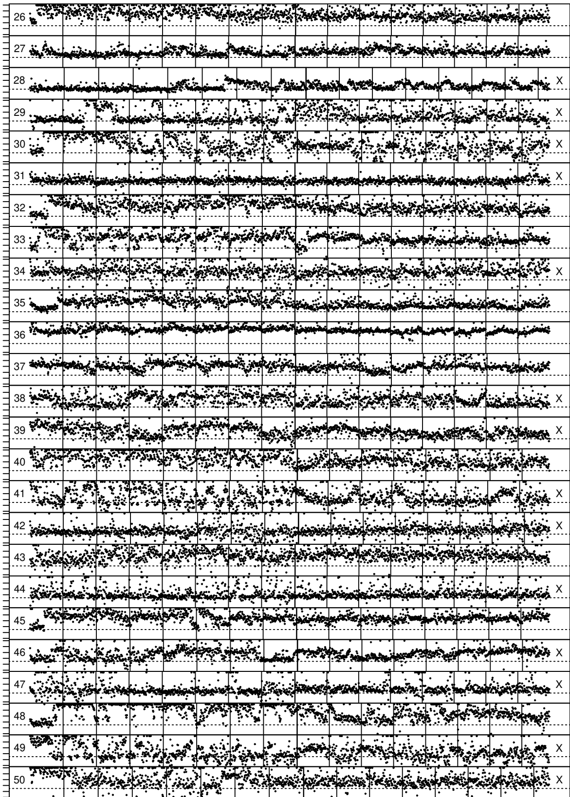
A time series plot of all RTs for all subjects in Experiment 2
