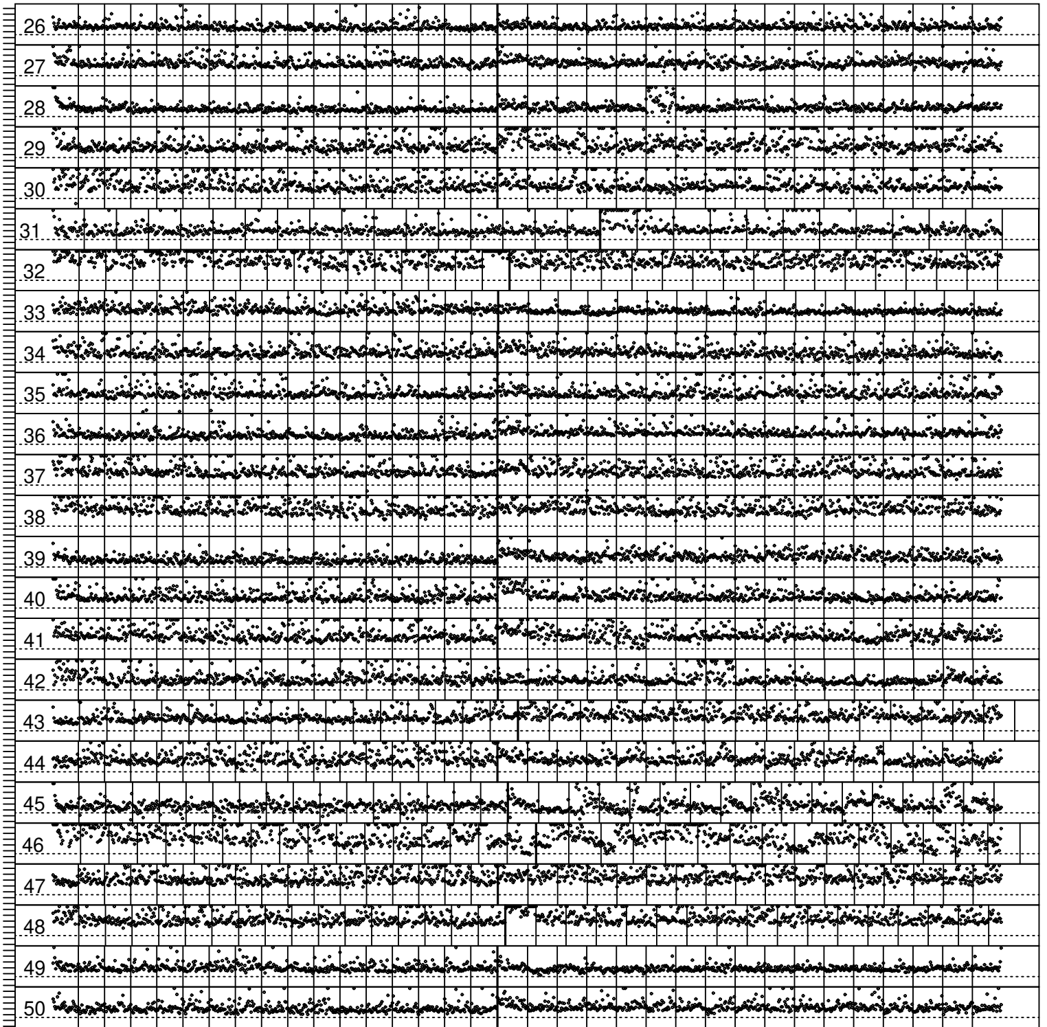
A time series plot of all RTs for all subjects in Experiment 1
