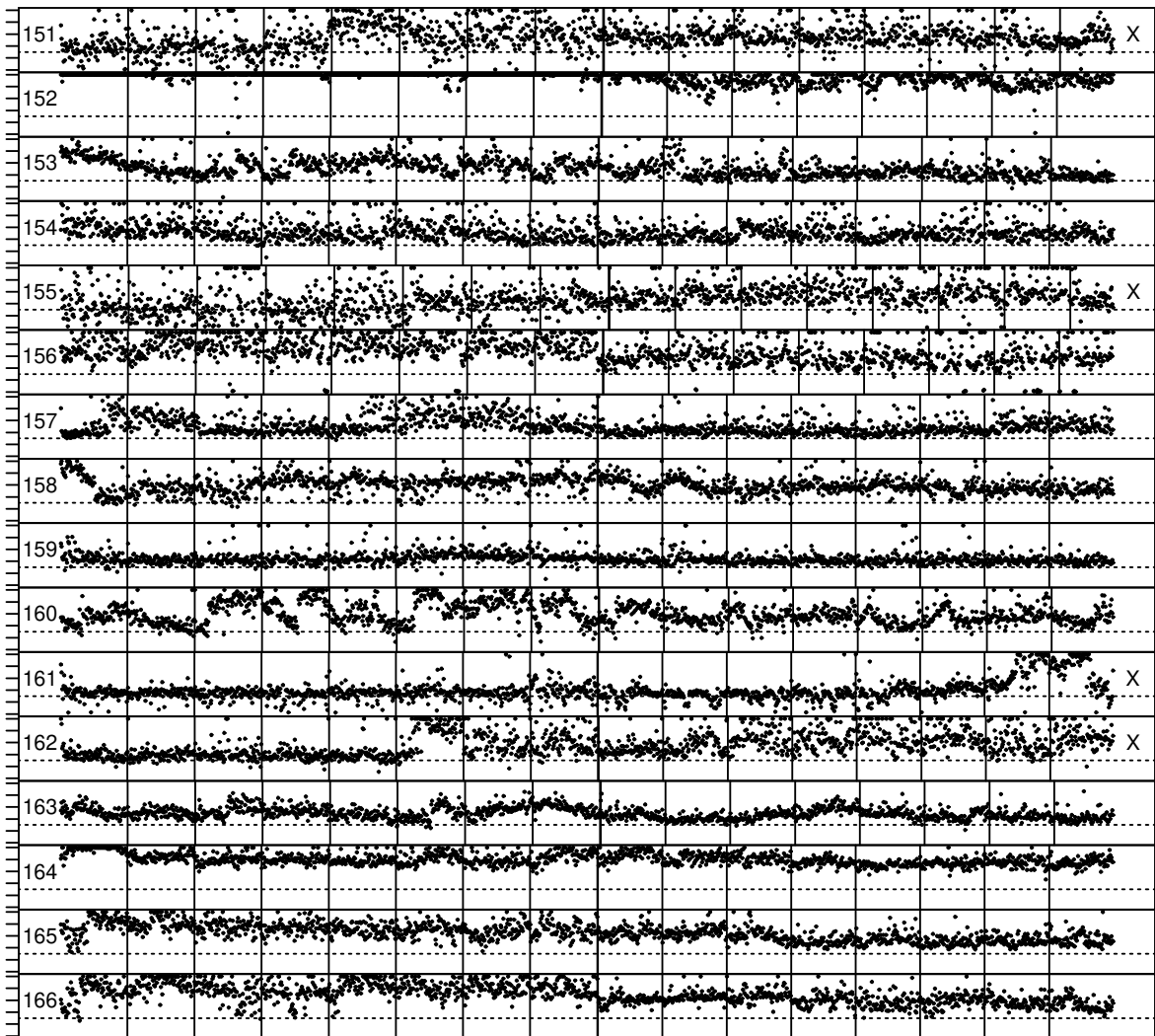
A time series plot of all RTs for all subjects in Experiment 2
