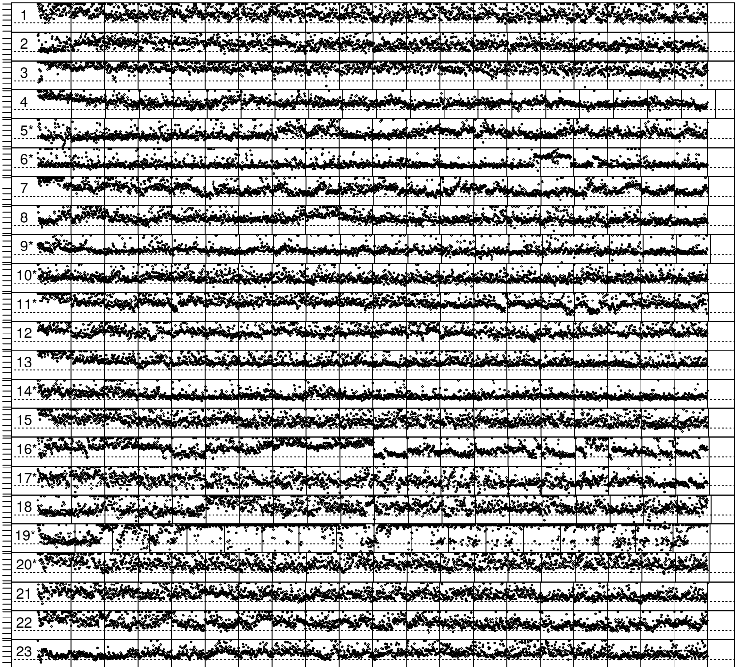
A time series plot of all RTs for all subjects for the BY task in Ratcliff & McKoon (2018)
