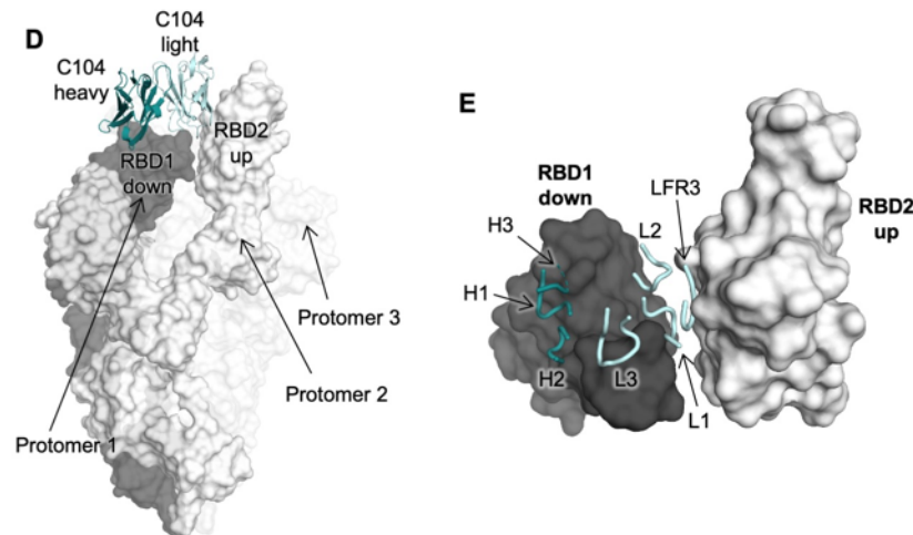
Figure S2. CDR H3 clusters 14 and 17 represent antibodies that bridge two RBDs in the same spike trimer. (A-C) Molecular feature of IGHV3-53/3-66 IGLV2-14 antibodies (cluster 14) that bridges two down RBDs simultaneously in a spike trimer. Cluster 14 contains 19 antibodies from 3 donors. (A) An overall view of SARS-CoV-2 spike in complex with an IGHV3-53/3-66 IGLV2-14 antibody. C144 (PDB 7K90) is used as a representative antibody [1]. Three protomers of the spike trimer are shown in charcoal, white, and transparent white, respectively. Heavy and light chains of C144 are shown in orange and yellow, respectively, with CDR H3 highlighted in red. The two RBDs bridged by the antibody are indicated in the figure. (B) Sequence logo of CDR H3 of IGHV3-53/3-66 IGLV2-14 antibodies, with residue positions labeled according to Kabat
