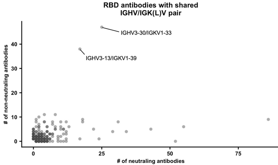
Figure S3. Identification of IGHV/IGK(L)V pairs that are enriched in non-neutralizing RBD antibodies. Each data point represents a defined IGHV/IGK(L)V pair. For each IGHV/IGK(L)V pair, the number of neutralizing RBD antibodies is plotted against the number of non-neutralizing RBD antibodies. Two IGHV/IGK(L)V pairs with a large number of non-neutralizing antibodies are labeled.
