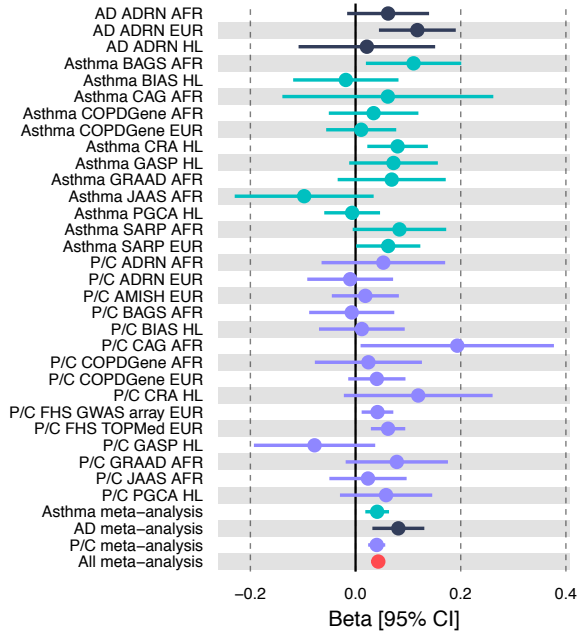
chr15q22.2 rs1059513
