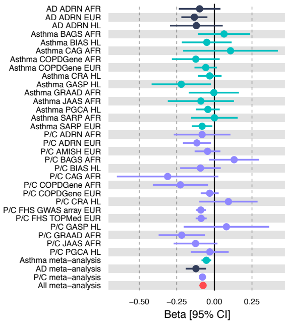
chr6p21.32 rs3104371
