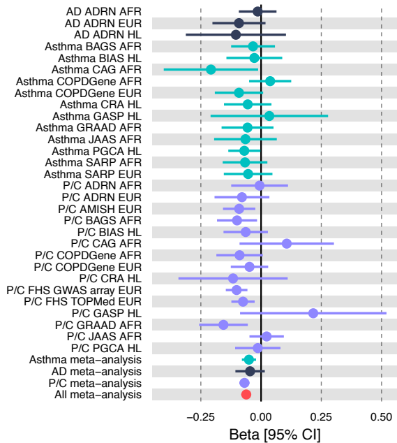
chr15q22.2 rs1059513
