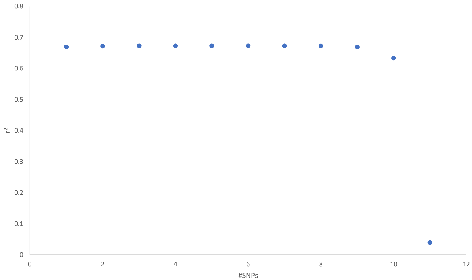
Figure S9. Lactase persistence r^2 maximization.
