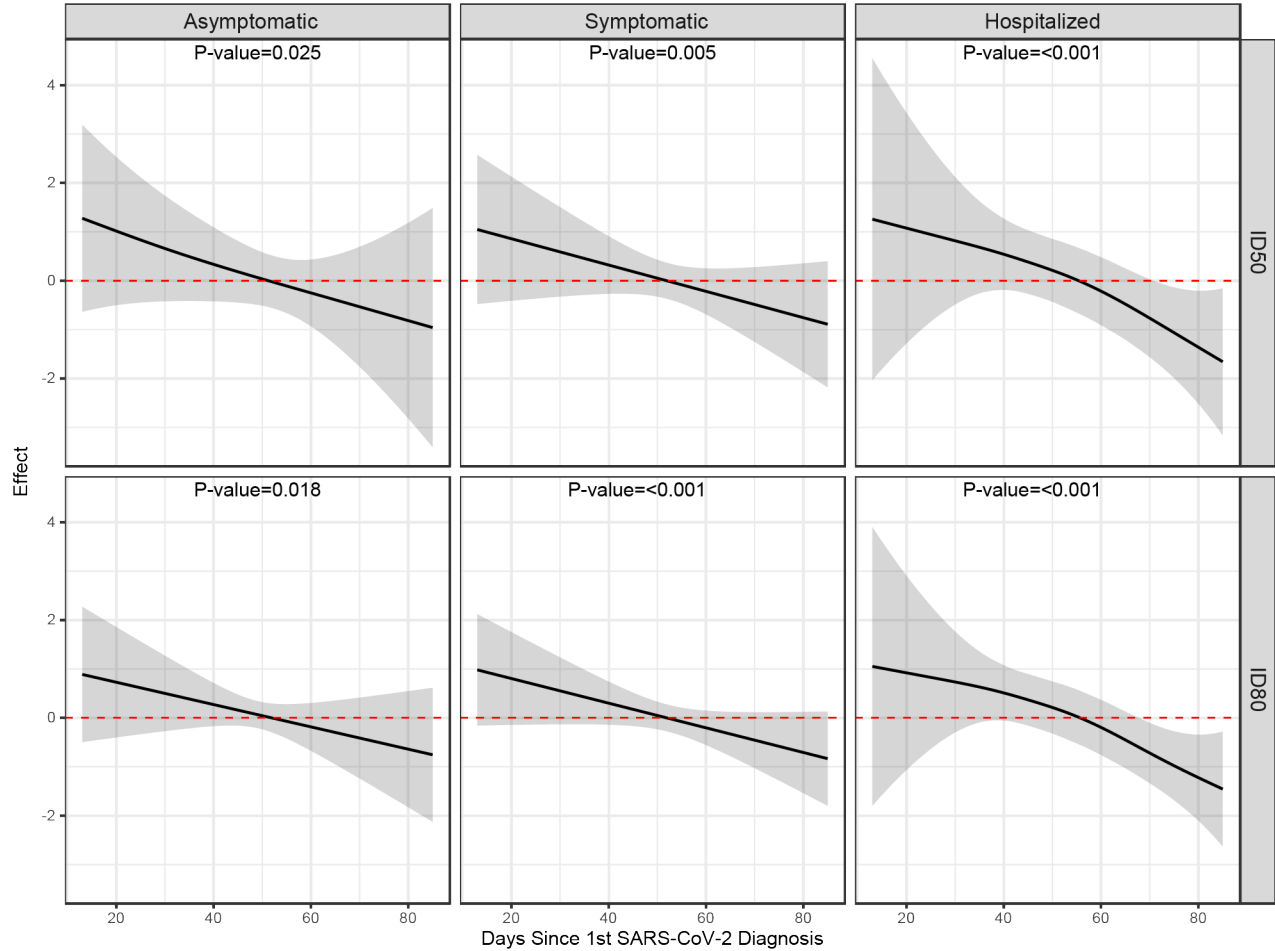
Figure D. Estimated days since SARS-CoV-2 diagnosis (days) effect on nAb log-titers stratifying by COVID-19 severity adjusting for COVID-19 severity, medical history, and demographics using generalized additive model.
