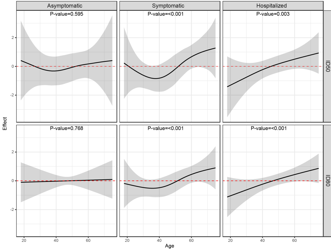
Figure B. Estimated age effect on nAb log-titers stratifying by COVID-19 severity adjusting for COVID-19 severity, medical history, other demographics, and days since SARS-CoV-2 diagnosis using generalized additive model.
