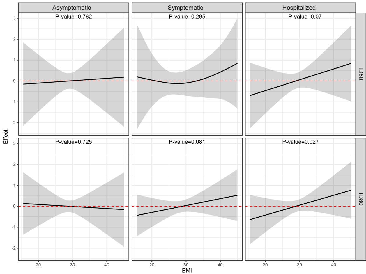
Figure E. Estimated BMI effect on nAb log-titers stratifying by COVID-19 severity adjusting for COVID-19 severity, medical history, other demographics, and days since SARS-CoV-2 diagnosis using generalized additive model.
