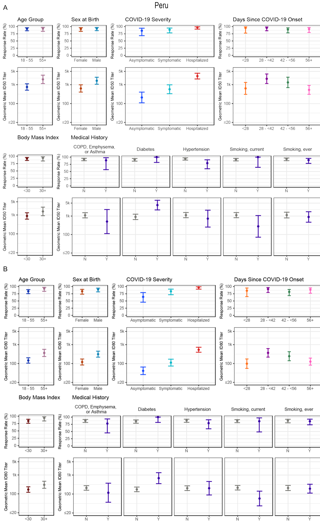
Figure F. Geometric mean titer (GMT) at enrollment visit and 95% CI by enrollment group, severity, medical history, and days since SARS-CoV-2 diagnosis in USA and Peru. A. Peru, ID50. B. Peru, ID80. C. US, ID50. D. US, ID80.
