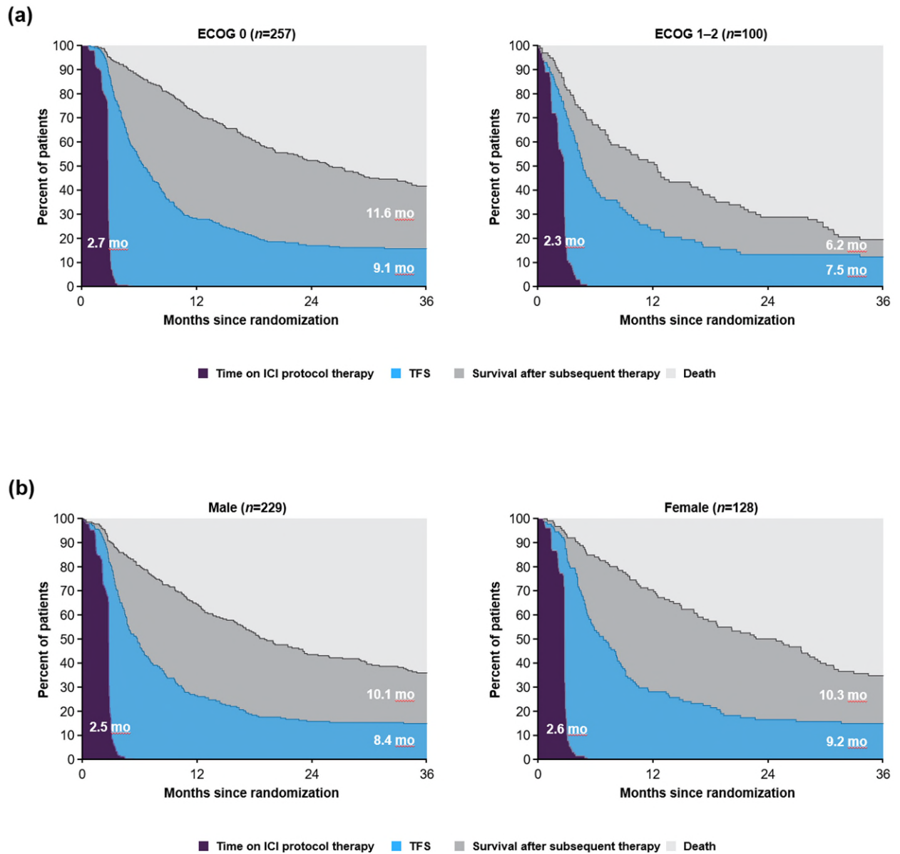
Fig. S3. Estimates of TFS and other health states over the 36-month period in patient subgroups based on (a) ECOG performance status and (b) sex in patients treated with ipilimumab. ECOG, Eastern Cooperative Oncology Group; ICI, immune checkpoint inhibitor; TFS, treatment-free survival.
