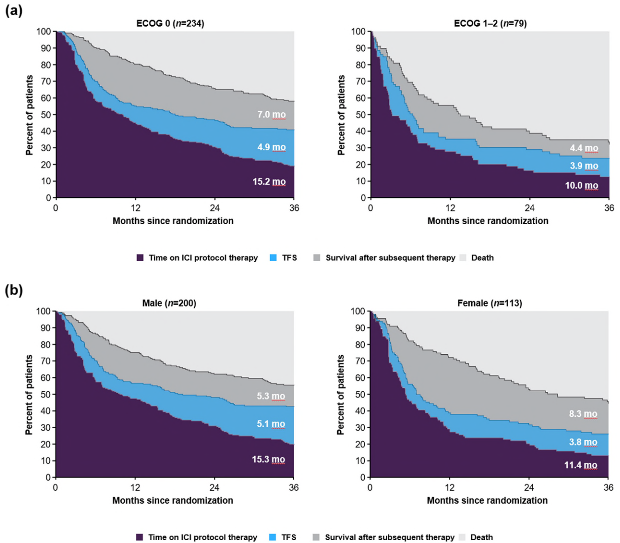
Fig S2. Estimates of TFS and other health states over the 36-month period in patient subgroups based on (a) ECOG performance status and (b) sex in patients treated with nivolumab. ECOG, Eastern Cooperative Oncology Group; ICI, immune checkpoint inhibitor; TFS, treatment-free survival.
