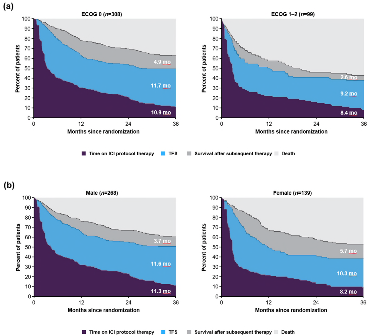
Fig. S1. Estimates of TFS and other health states over the 36-month period in patient subgroups based on (a) ECOG performance status and (b) sex in patients treated with nivolumab plus ipilimumab. ECOG, Eastern Cooperative Oncology Group; ICI, immune checkpoint inhibitor; TFS, treatment-free survival.
