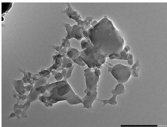
Figure S1. TEM image of Cu 3 (BTC) 2
