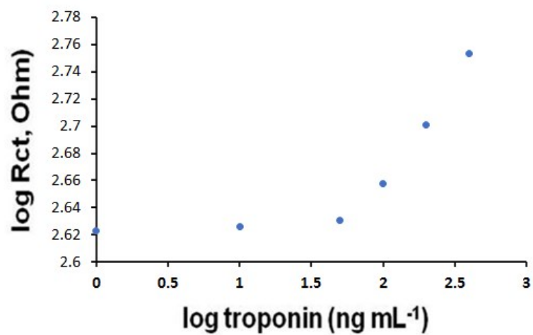
Figure S2. Detection of cTnI with a reference Ab/PANI biosensor, the sensor did not produce any discernible response below 50 ng/mL
