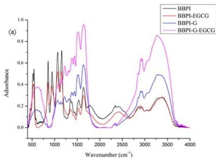
Supplementary Fig. S2 (a) is FTIR of BBPI, BBPI-EGCG, BBPI-G-EGCG, BBPI-G-EGCG. (b) is peak fitting image of BBPI. (c) is peak fitting image of BBPI-EGCG. (d) is peak fitting image of BBPI-G. (e) is peak fitting image of BBPI-G-EGCG.
