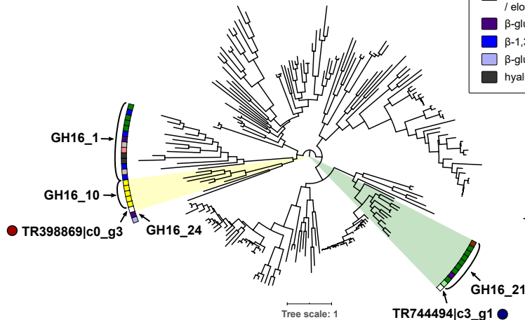
Mixed-linkage glucan
