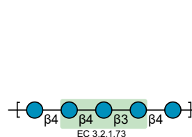
Mixed-linkage glucan
