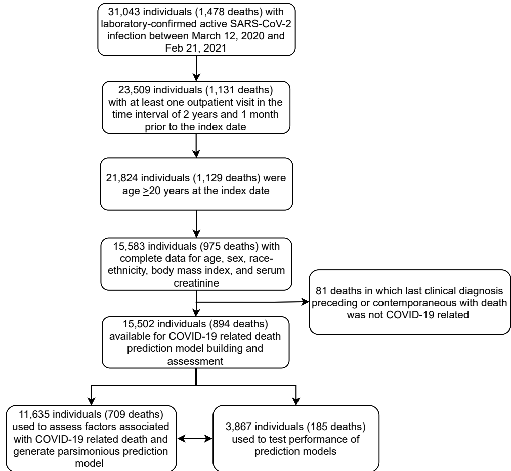
Figure S1. Flow chart demonstrating how the final analytic set of individuals with laboratory confirmed SARS-CoV-2 was selected, as well as the numbers used for prediction model development and testing.
