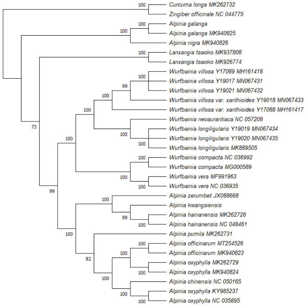
Supplementary Figure 3 Phylogenetic tree constructed using maximum likelihood (ML) based on the 32 complete CP genomes. Numbers above the branches are the bootstrap support values.
