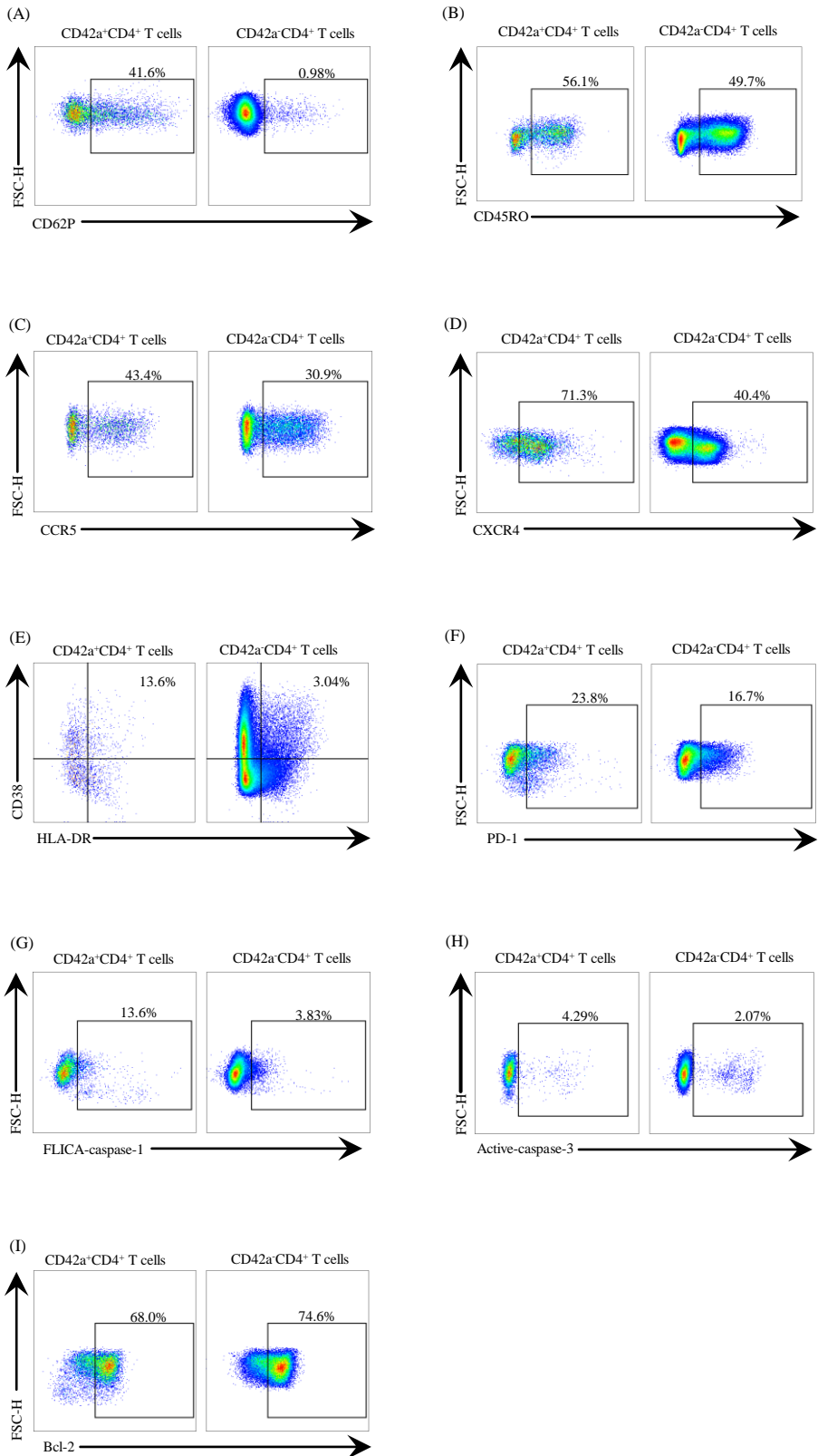
Supplementary Figure 1. Detection of phenotypic characteristics of platelet-CD4 + T cell aggregates. Representative gating strategy for CD62P (A), CD45RO (B), CCR5 (C), CXCR4 (D), HLA-DR/CD38 (E), PD-1 (F), FLICA-caspase-1 (G), Active-caspase-3 (H), and Bcl-2 (I) expression in platelet-CD4 + T cell aggregates and their counterparts.
