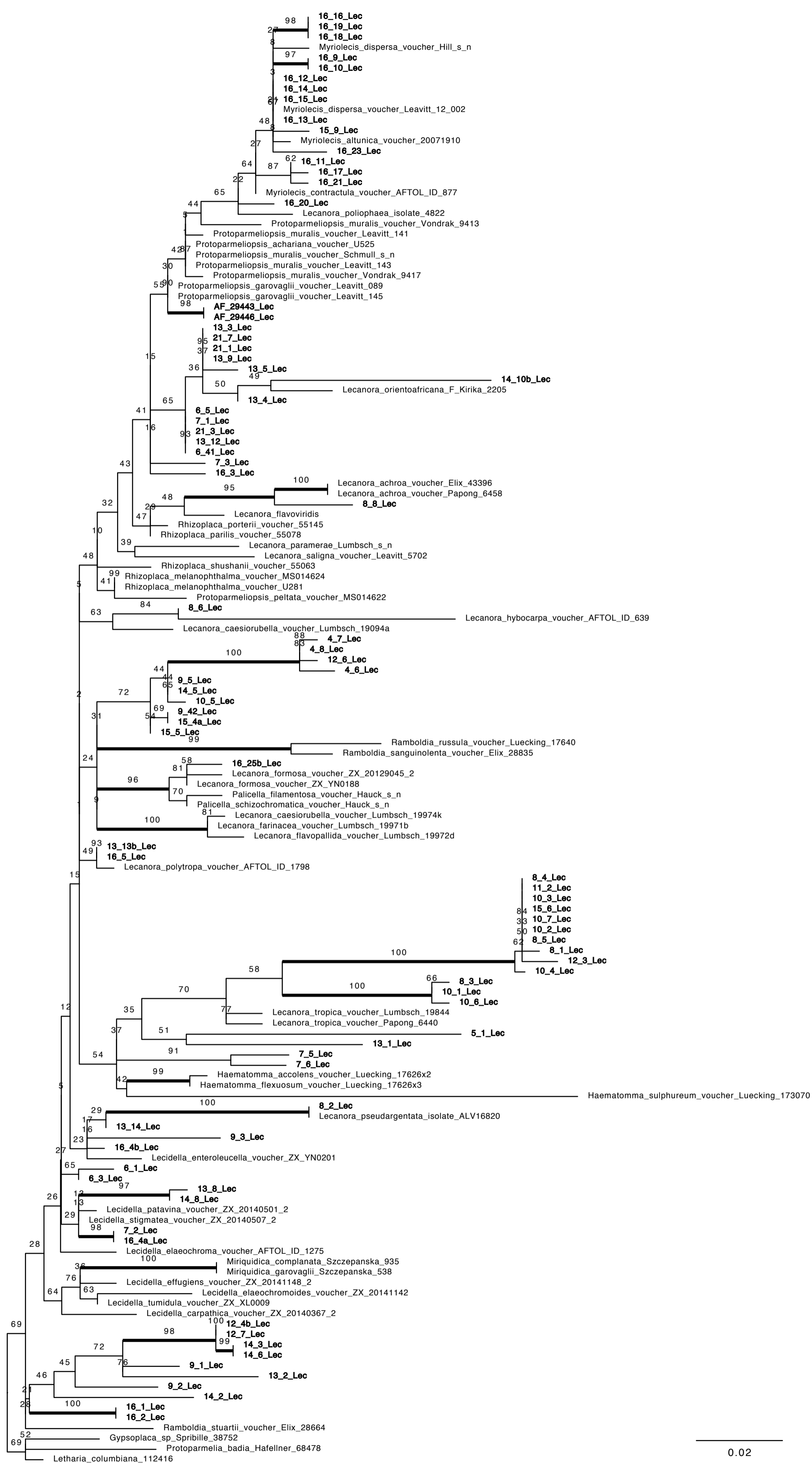
Supplementary figure 6. Single-locus tree for Lecanoraceae ITS. Maximum-likelihood tree inferred with the K2P+R3 substitution model. Support values are UFboot2 with 5000 replicates. Bipartitions with bootstrap support \geq 95 are indicated with bold branches. Bold tip names indicate specimens sequenced in this study. Scale indicates substitutions per site.
