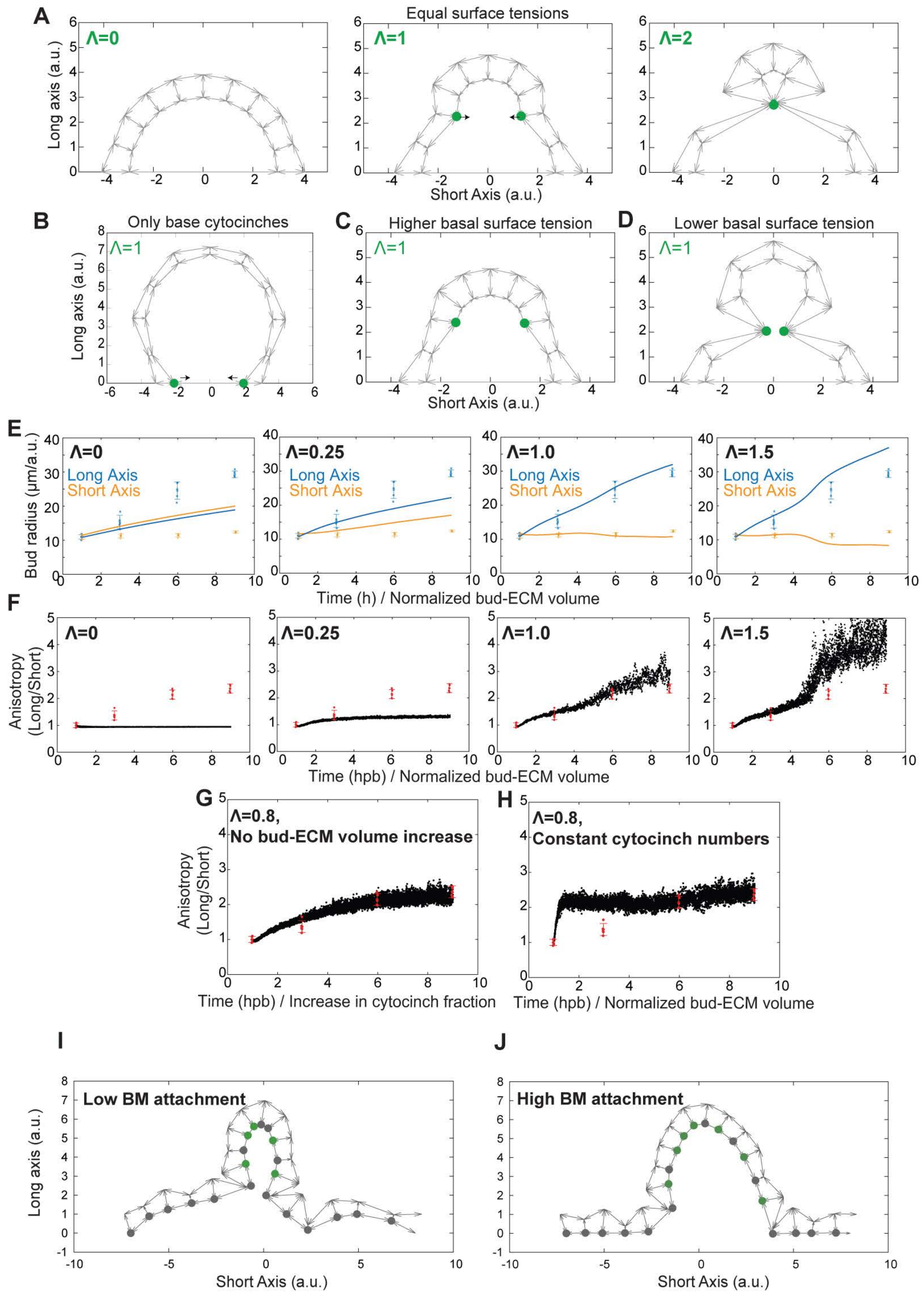
Figure S5 (Related to Figure 7) - A vertex model for bud-to-tube morphogenesis
