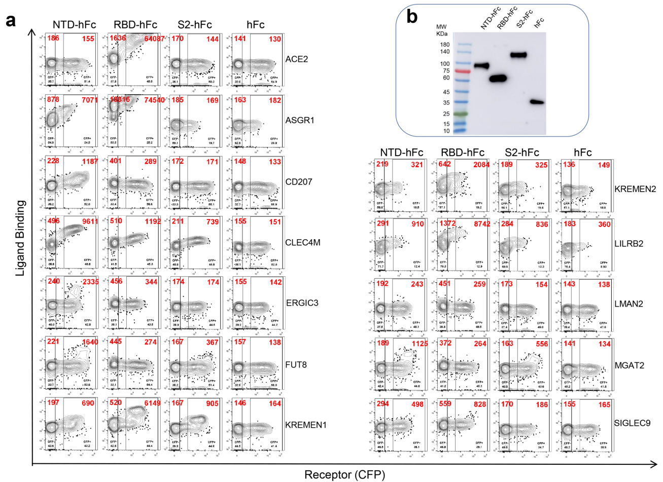
Fig. S2. Binding of the identified host factors with SARS-CoV-2 spike domains.
