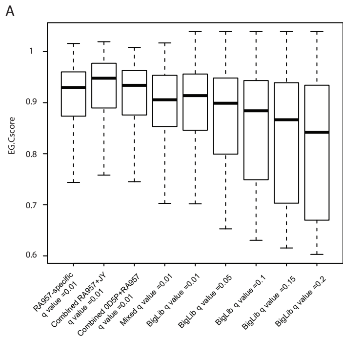
Supplemental Figure 4: EG.Cscore distributions ( A ) and differences between the predicted RT= f(iRT) and the mean measured RT ( B ) in RA957 DIA data in relation to the library size (RA957 sample specific, combined, mixed, and BigLib, as well as BigLib analyzed with increasing q values).
