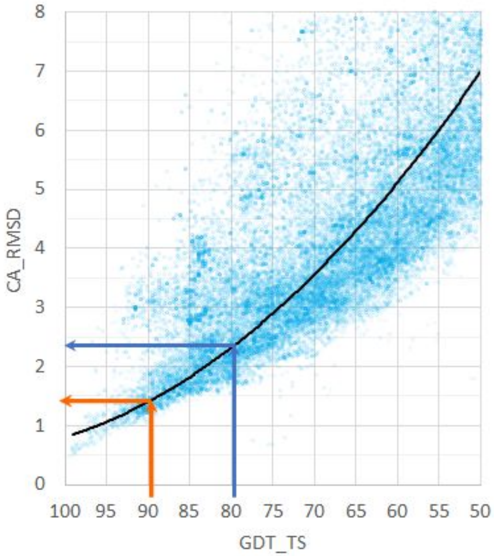
Figure S1: Relationship between C \alpha RMSD and GDT_TS for higher accuracy CASP14 models.
