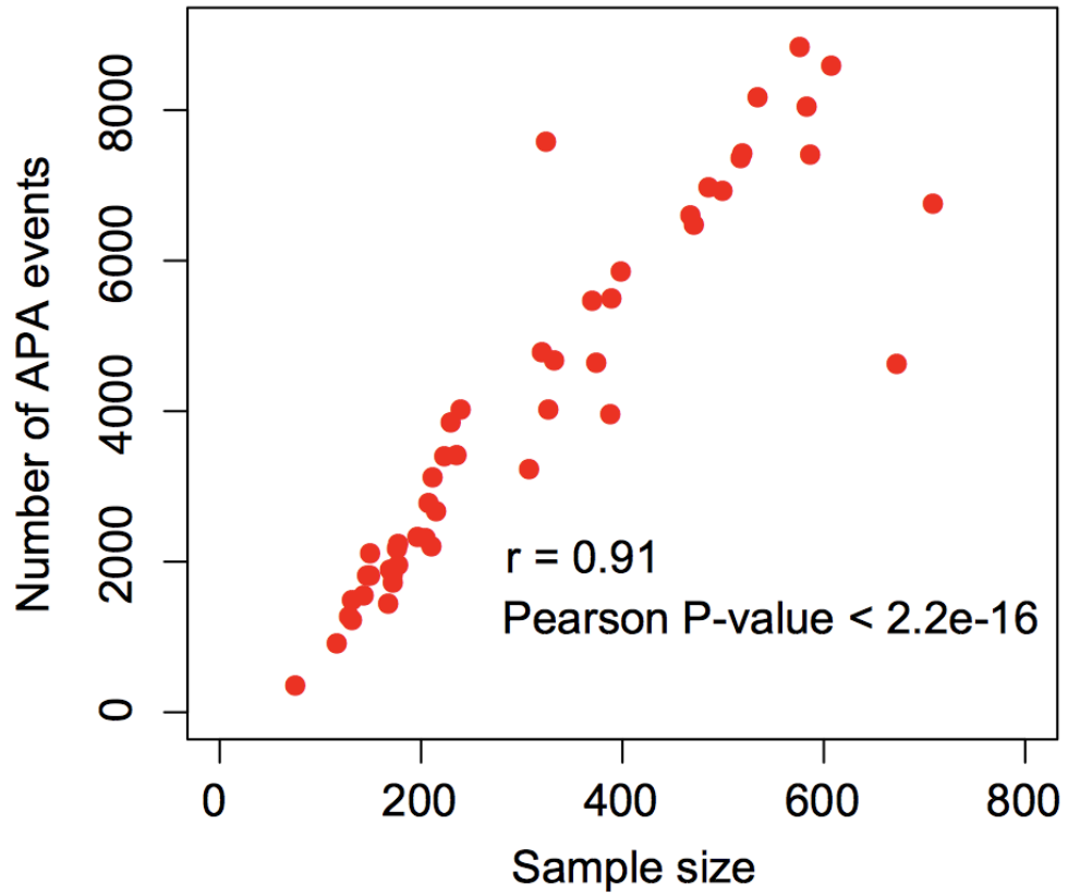
Supplementary Figure S1. The number of 3'aQTL APA events was highly correlated (Pearson correlation P-value < 2.2e-16 , r=0.91 ) with the sample size in each tissue. Each dot indicates a tissue type.
