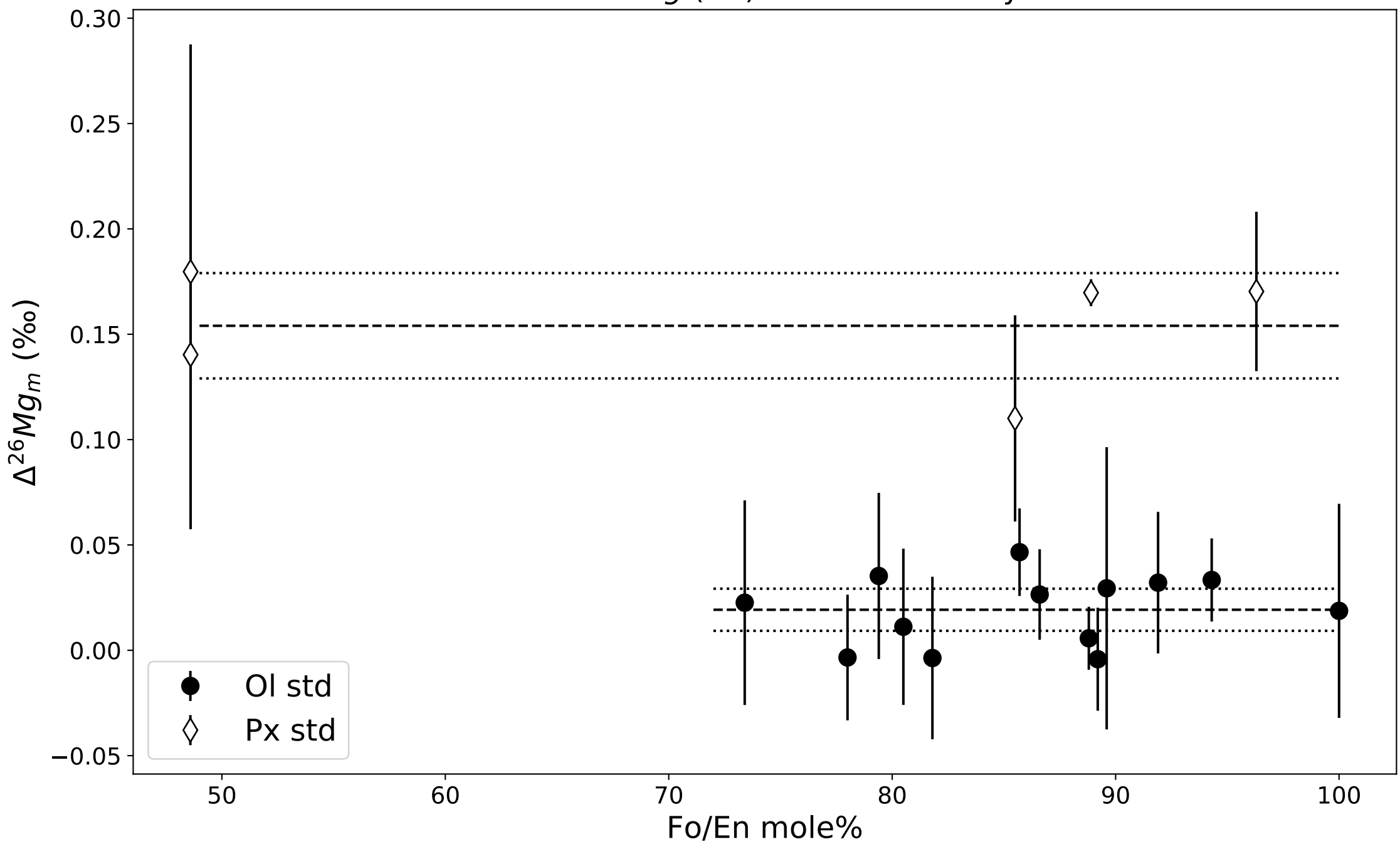
Determination of the exponential factor \beta using terrestrial Olivine standards
