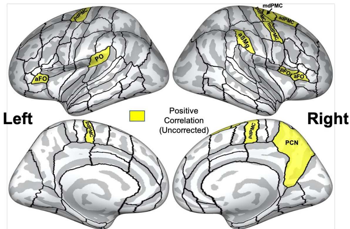
Supplemental Figure S6. Exploratory regions-of-interest (ROIs) with a positive correlation between normal – baseline activation and SSI-Mod in AWS ( p < .05 ) are highlighted in yellow and plotted on an inflated cortical surface. Black outlines indicate cortical ROIs used in the exploratory analysis. adPMC = anterior dorsal premotor cortex, aFO = anterior frontal operculum, aSMg = anterior supramarginal gyrus, mdPMC = middle dorsal premotor cortex, PCN = precuneus, pdPMC = posterior dorsal premotor cortex, pFO = posterior frontal operculum, PO = parietal operculum.
