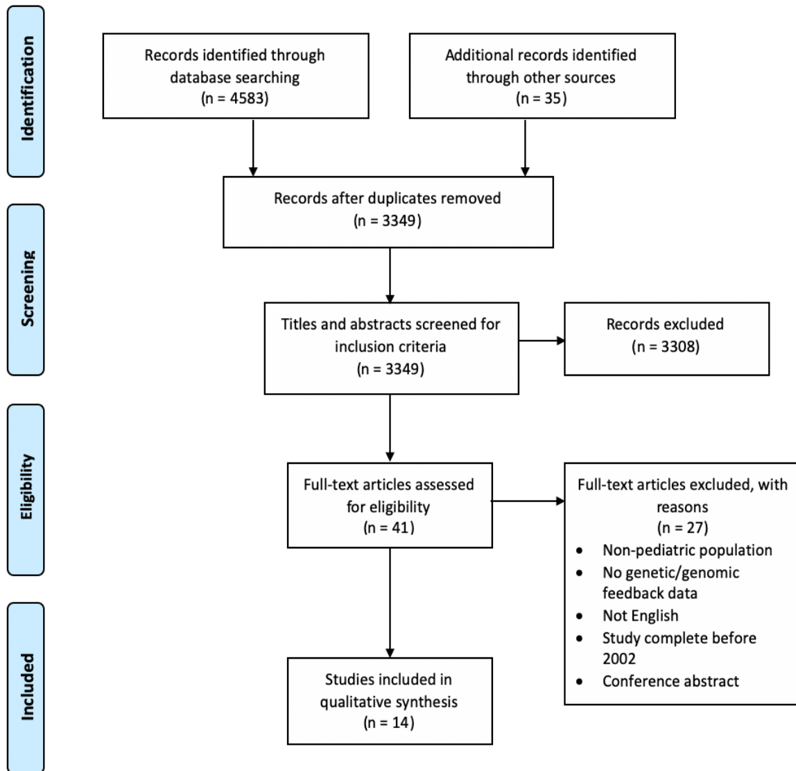
Figure 2. Prisma diagram
