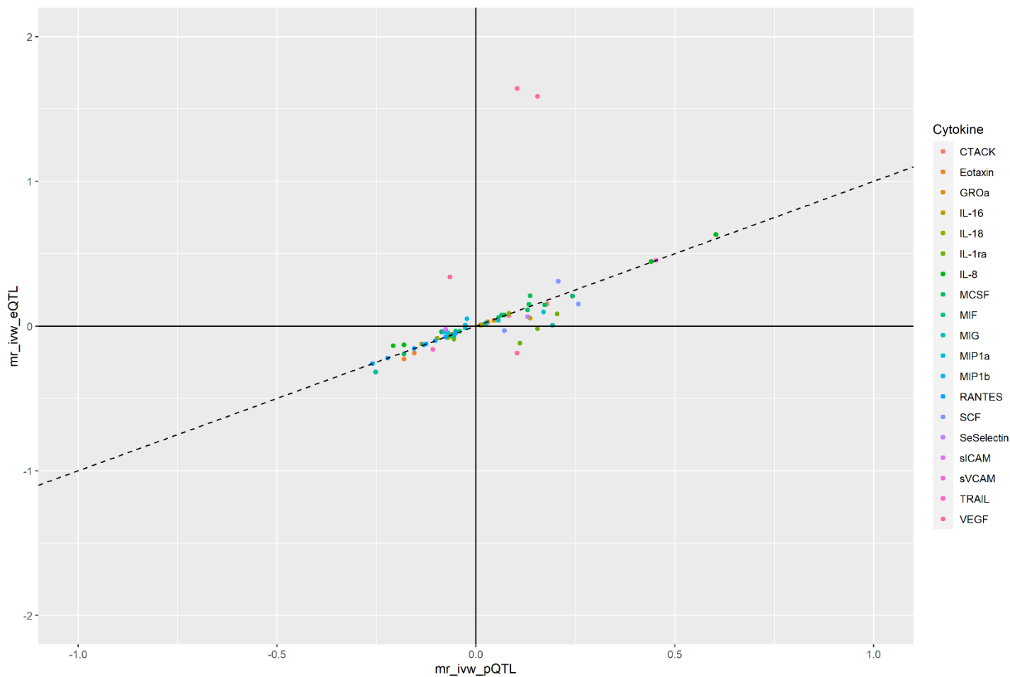
Supplementary figure 1. Correlation of MR-IVW estimates (betas) using the two different instrument definitions. Y axis represents the MR IVW estimates using the cis-eQTL and X axis represents the MR IVW estimates using the cis-pQTL instrument definition.
