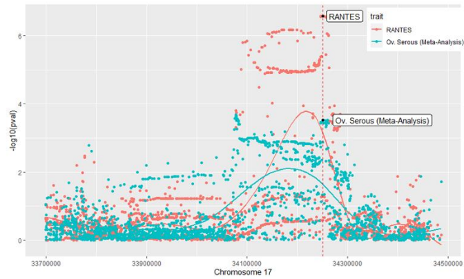
Supplementary figure 2. Associations that showed MR evidence for both causality and colocalization (posterior probability > 0.8) are plotted, within \pm 500 kb of the gene locus of the exposure cytokine.
