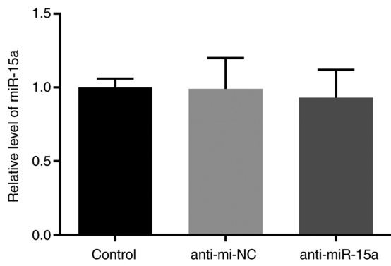
Figure S1. Transfection with miR-15a inhibitor has no effect on miR-15a expression. Reverse transcription-quantitative PCR analysis was performed to detect the effect of transfection with miR-15a inhibitor and anti-mi-NC on miR-15a expression in LNCAP cells. miR, microRNA; NC, negative control.
