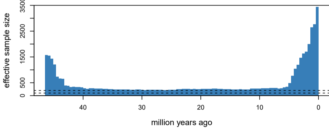
extinction rates
