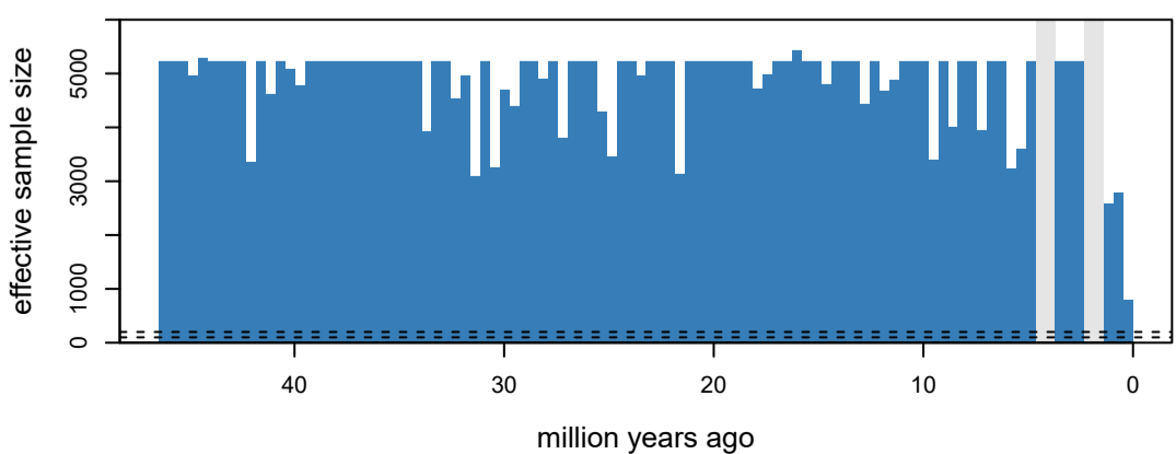
mass extinction times
