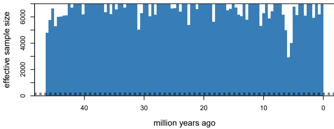
speciation shift times
