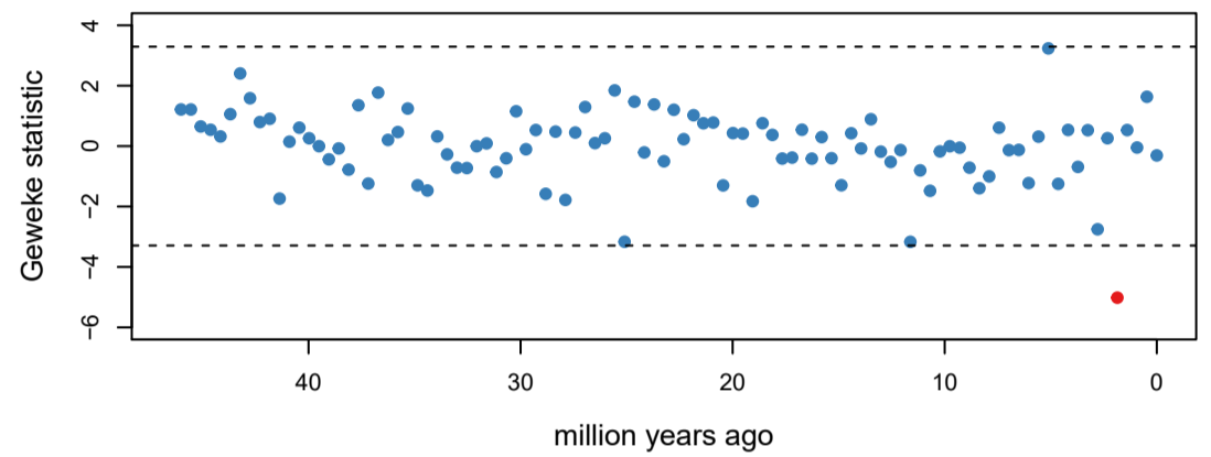
speciation shift times
