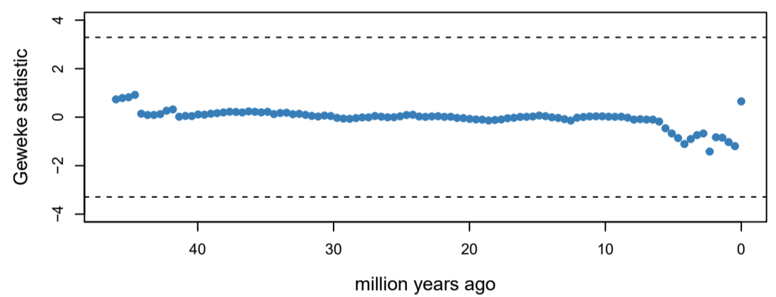
extinction rates
