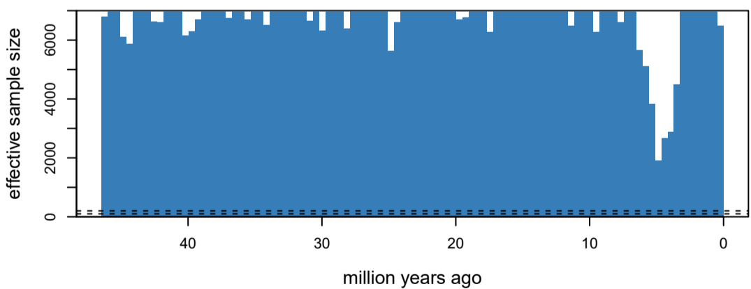
extinction shift times
