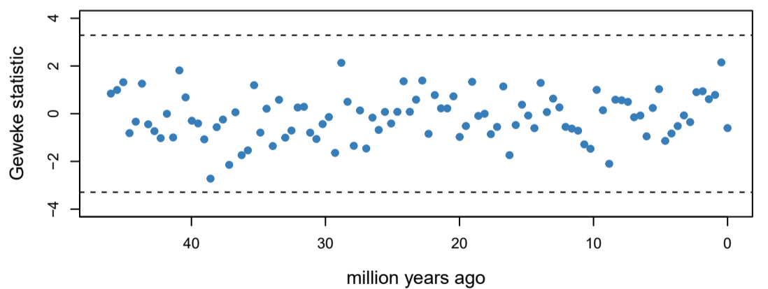
extinction shift times
