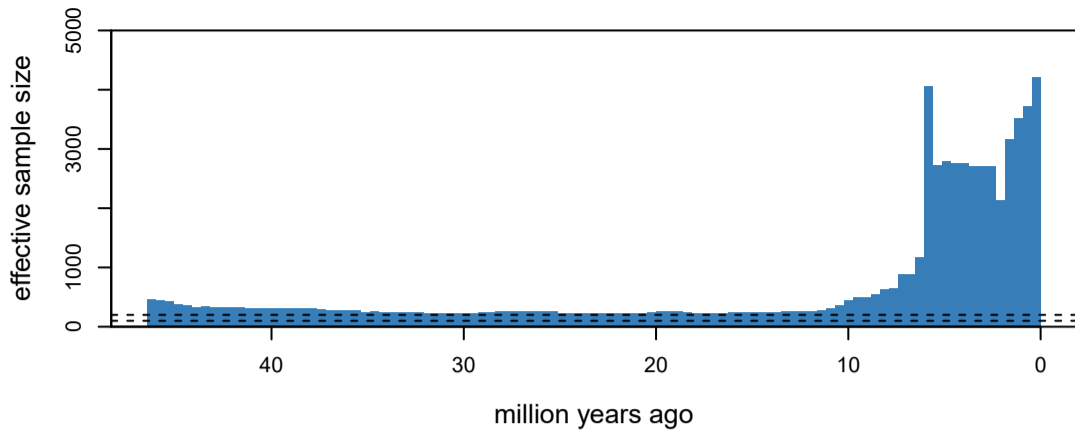
speciation rates
