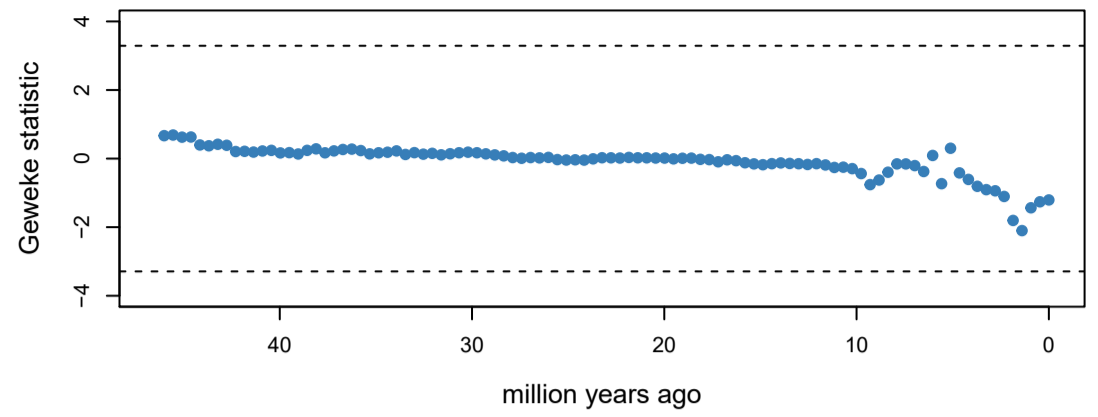
speciation rates
