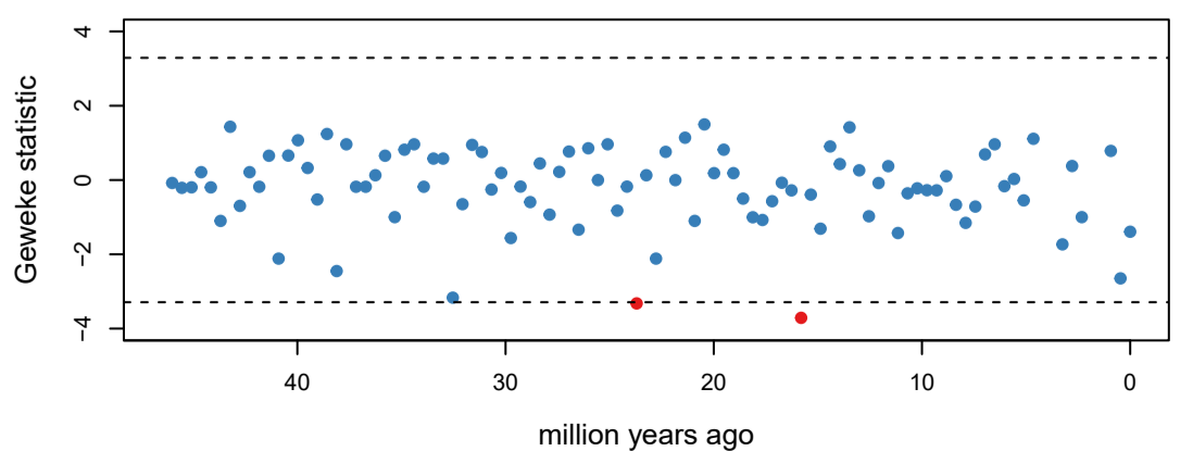
mass extinction times
