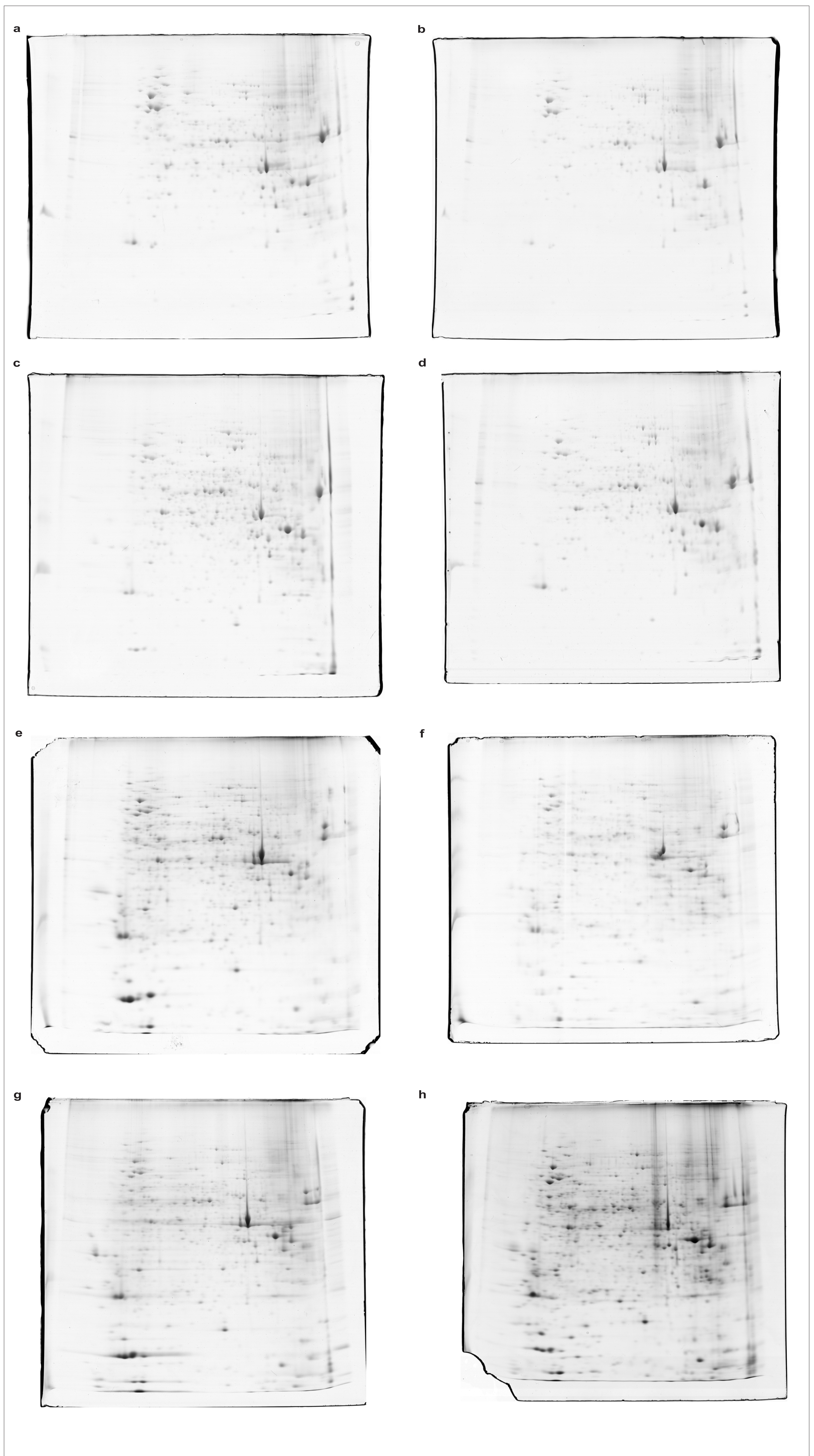
Supplementary figure 3: 2D gels of the protein profile of different stages of Mp infection in resistant and susceptible cocoa meristems . a: Catongo 72 HAI non -inoculated [mock inoculated control ] . b: Catongo 72 HAI. c: TSH1188 72 HAI non -inoculate d [mock inoculated control ] . d: TSH1188 72 HAI. e: Catongo 45 DAI non -inoculated [mock inoculated control ] . f: Catongo 45 DAI. g: TSH1188 45 DAI non -inoculated [mock inoculated control ] . h: TSH1188 45 DAI.
