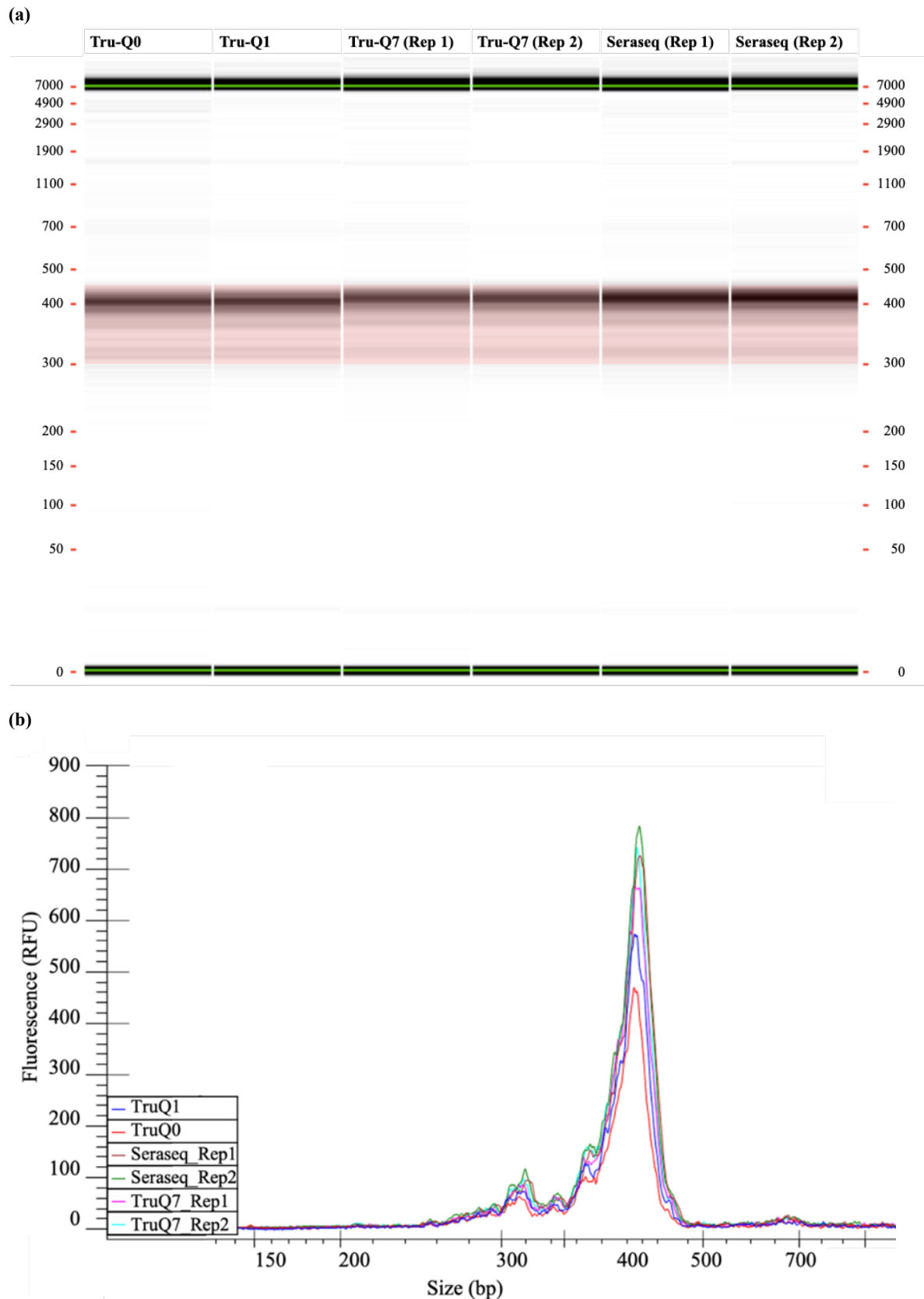
Additional file 5: Fig. S1. Representative image of (a) Labchip gel and (b) multiple overlay electropherogram of the constructed libraries of the reference standards. The image shows the quality and quantity of input DNA for the second NGS run for the technical validation of the custom NGS panel. The majority of the constructed libraries were within the targeted size range of 400 bp.
