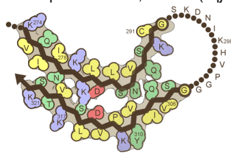
J 4R Tau heparin induced, Twister (6qjm)
