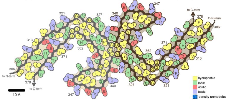
A Tau PHF filament from Alzheimer's disease brain (5o3L)
