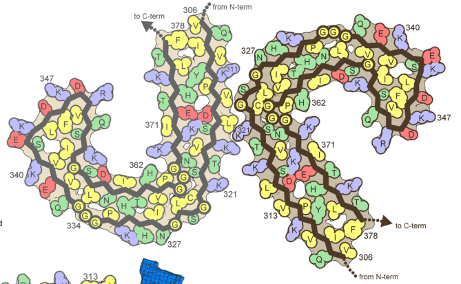
D Tau filament: chronic traumatic encephalopathy type II (6nwq)
