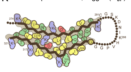
K 4R Tau heparin induced, Jagged (6qjp)
