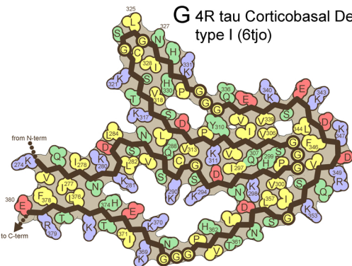
I 4R Tau heparin induced, Snake (6qjh)
