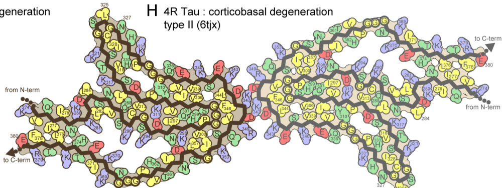
J 4R Tau heparin induced, Twister (6qjm)
