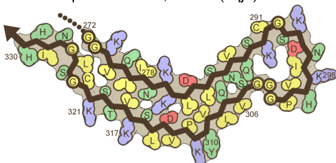
I 4R Tau heparin induced, Snake (6qjh)
