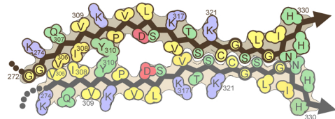
F Tau 3R heparin induced (6qjq)
