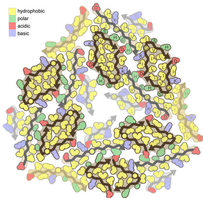
E TDP-43 RRM2 (247-257)(5w7v)
