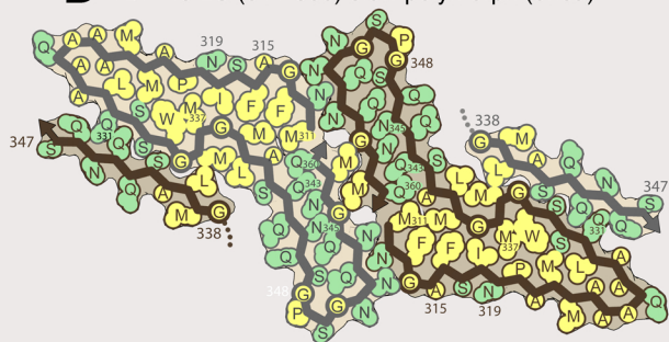
D TDP-43 LC (311-360) slow polymorph (6n3a)
