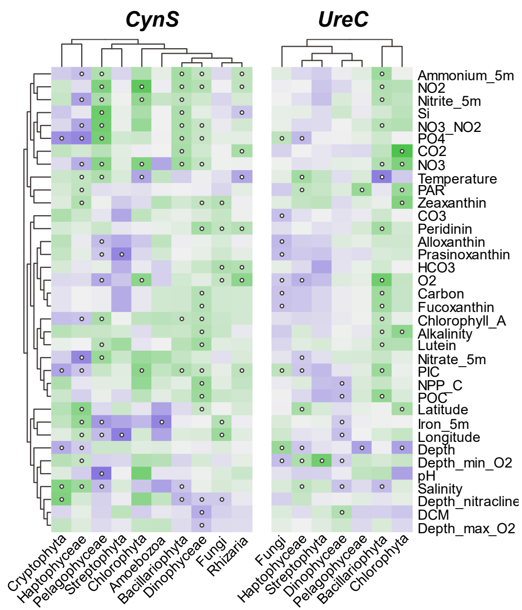
(a) Gene Expression (0.8-2000 \mu\text{m} fraction)
