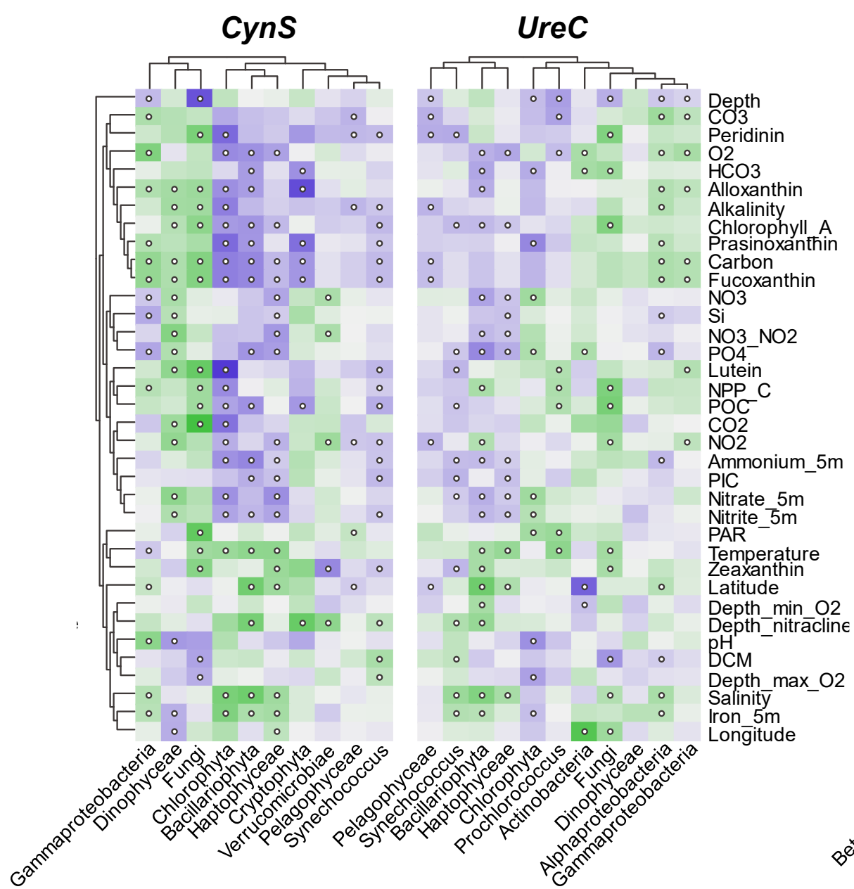
(c) Gene Abundance (0.8-2000 \mu\text{m} fraction)
