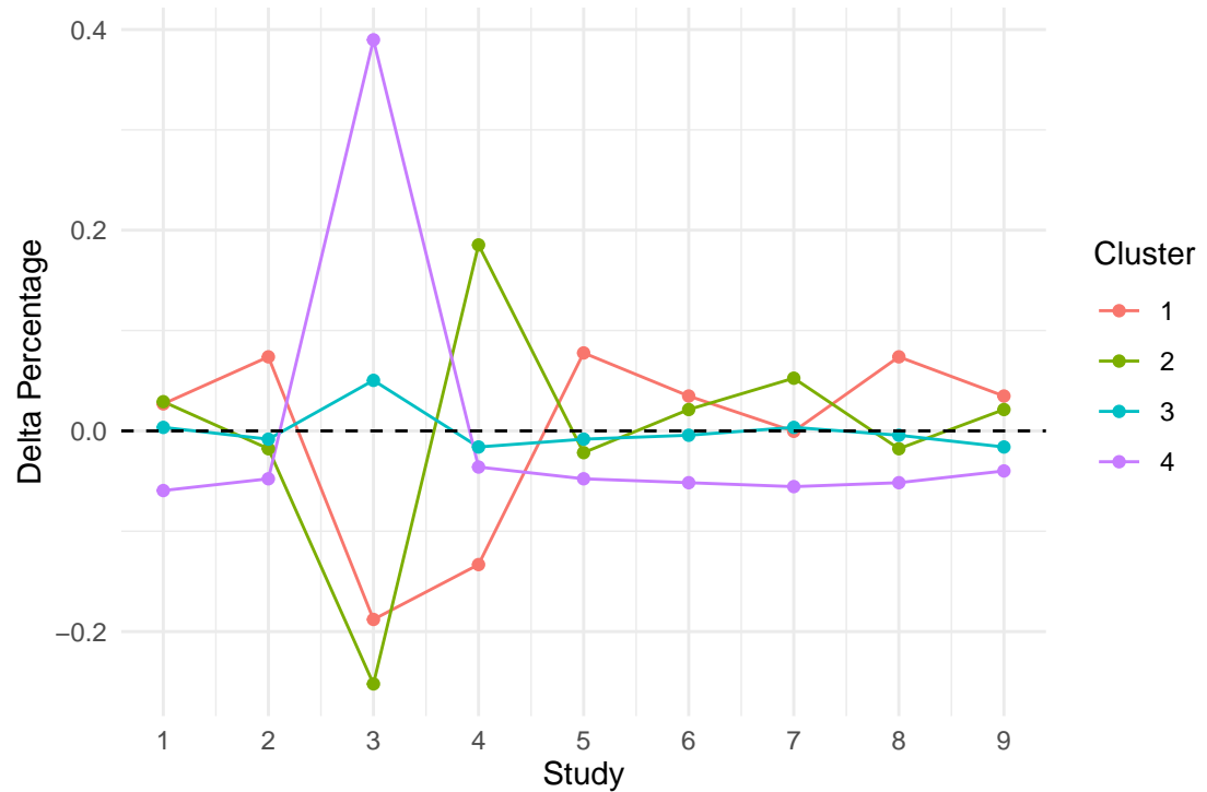
Cluster imbalance (Cook's Distance)
