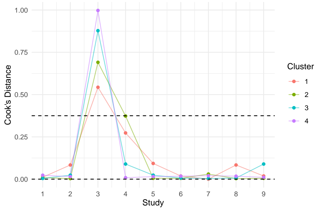
Cluster imbalance (Cook's Distance)
