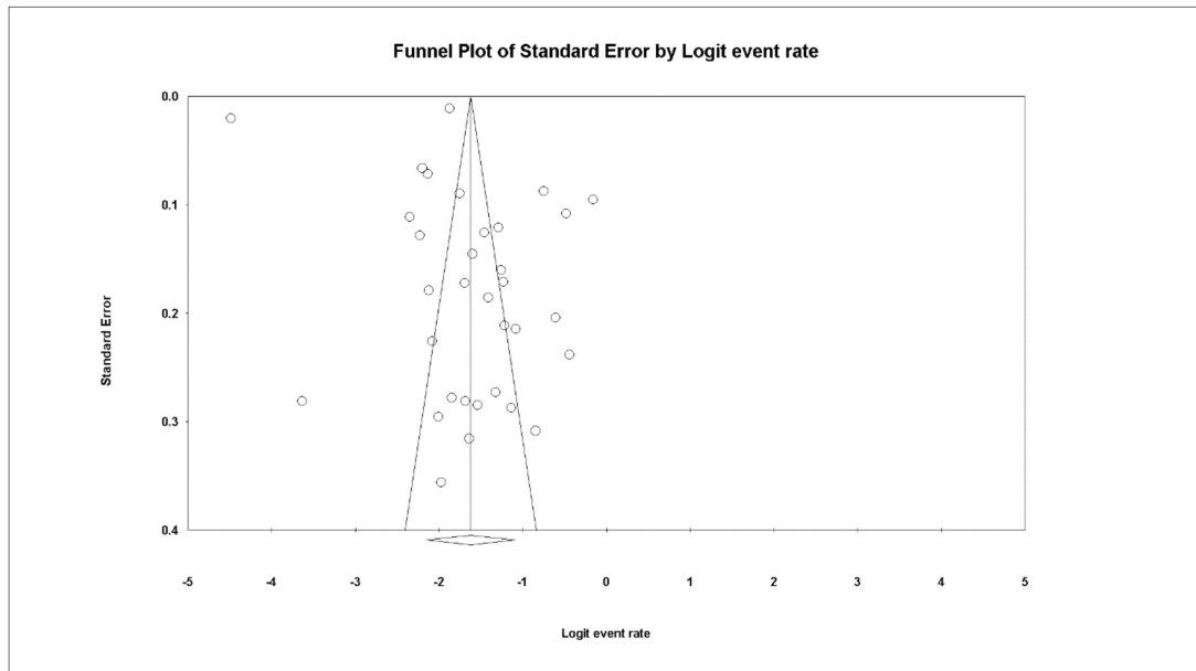
Figure S10 Funnel Plot (PSD all timeframes, excluding pre-stroke dementia)
