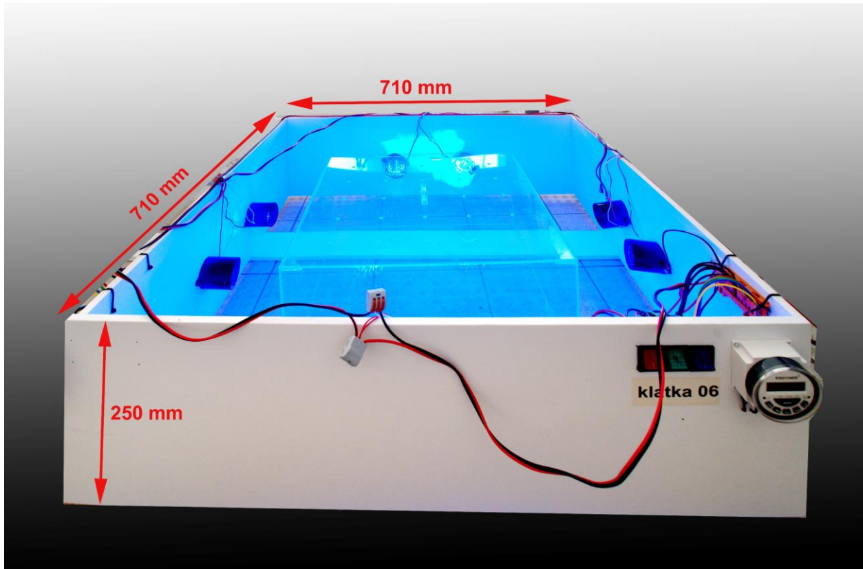
Supplementary Figure 1. Enclosure for experimental light exposure.
