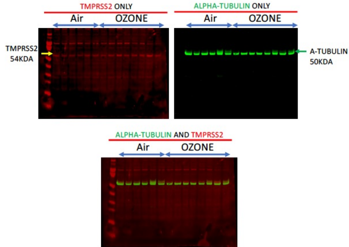
Supplementary Figure 1. Western blot gel image showing bands for TMPRSS2 protein on the whole lung homogenate from Air- and Ozone-exposed mice (n=6-8).
