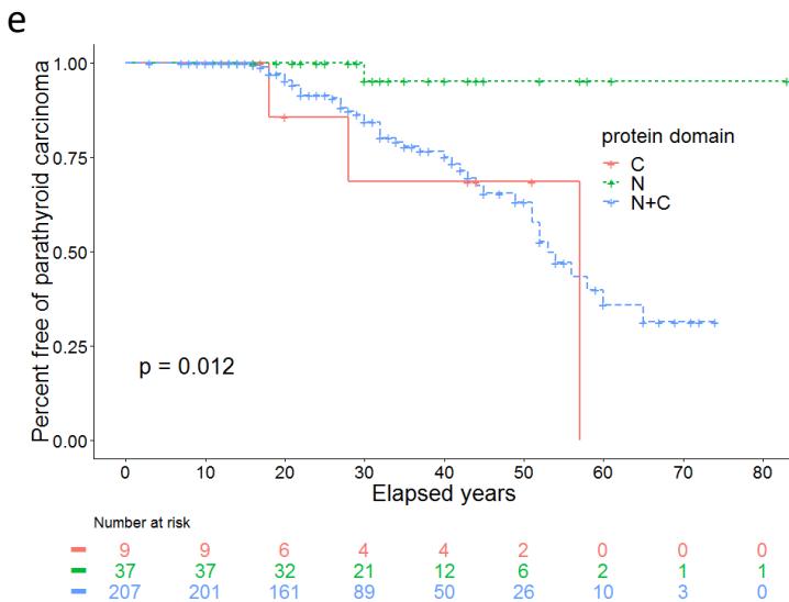
Supplementary Figure 5. Kaplan-Meier plots of event-free survival of parathyroid carcinoma (left) and hyperparathyroidism (right) in several subsets of the subjects grouped by the mutations affecting the NTD only (N), the CTD only (C) or both protein domains (N+C): (a,b) Subjects with sequencing-confirmed CDC73 germline mutations; (c,d) subjects who were index cases; and (e,f) subjects after atypical parathyroid adenomas were excluded.
