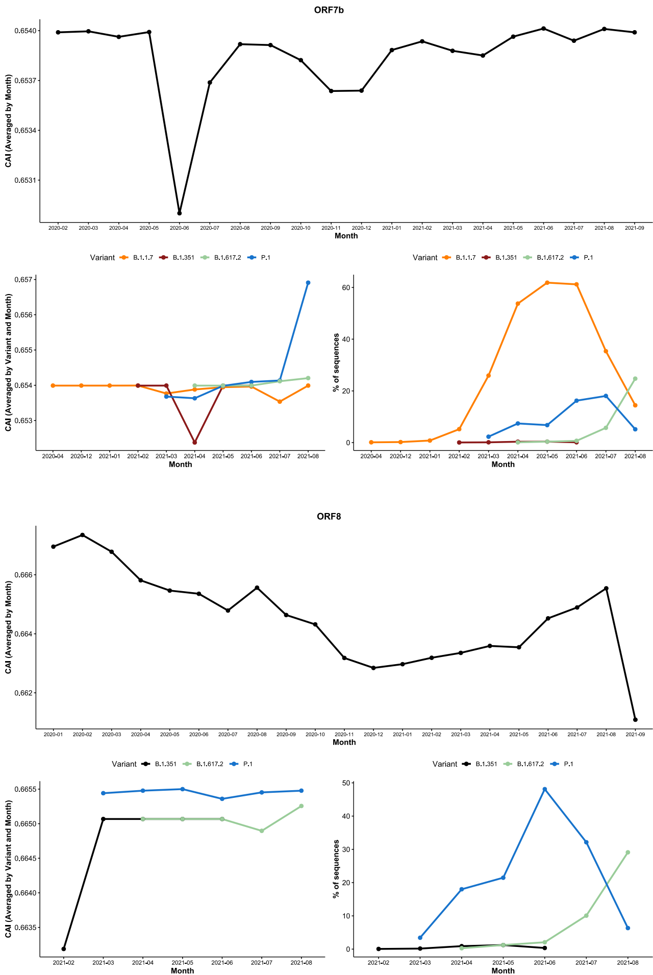
Figure S16. Evolution of CAI for SARSCoV2 ORFs over time for the California dataset.
