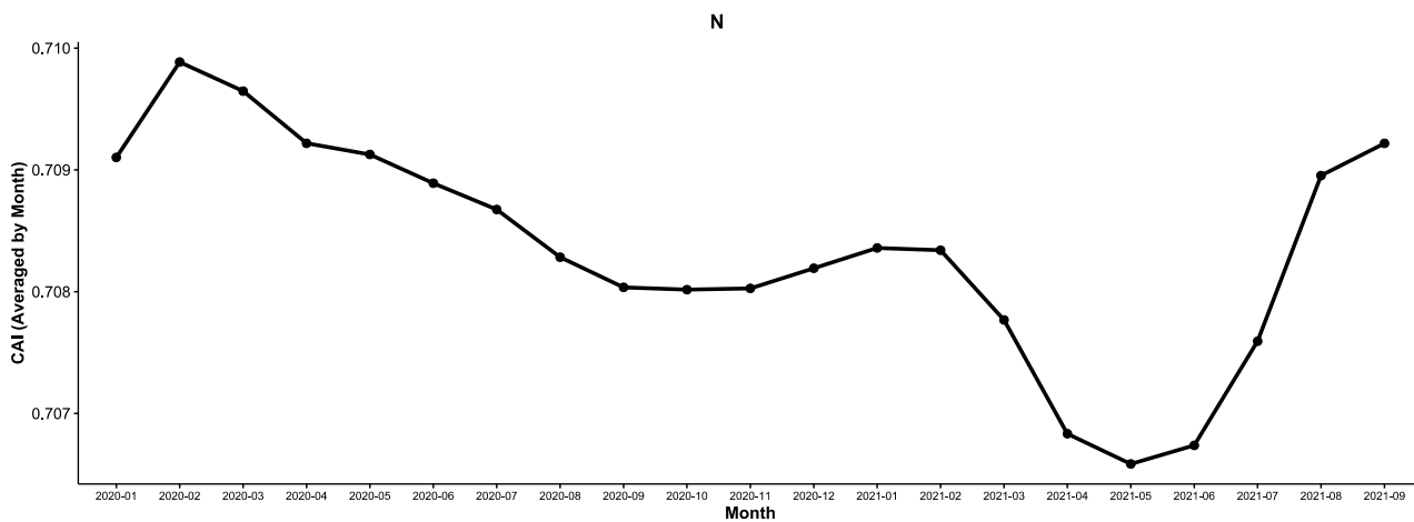
Figure S16. Evolution of CAI for SARSCoV2 ORFs over time for the California dataset.
