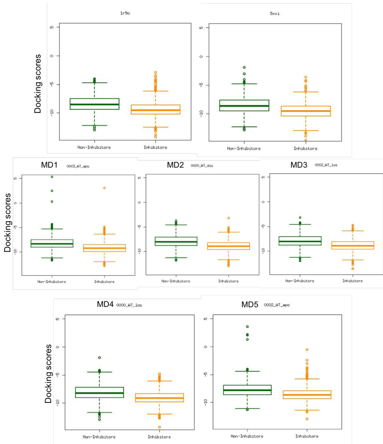
Figure S3. Autodock Vina scores of the training set' inhibitors and non-inhibitors calculated on seven different CYP2C9 conformations.
