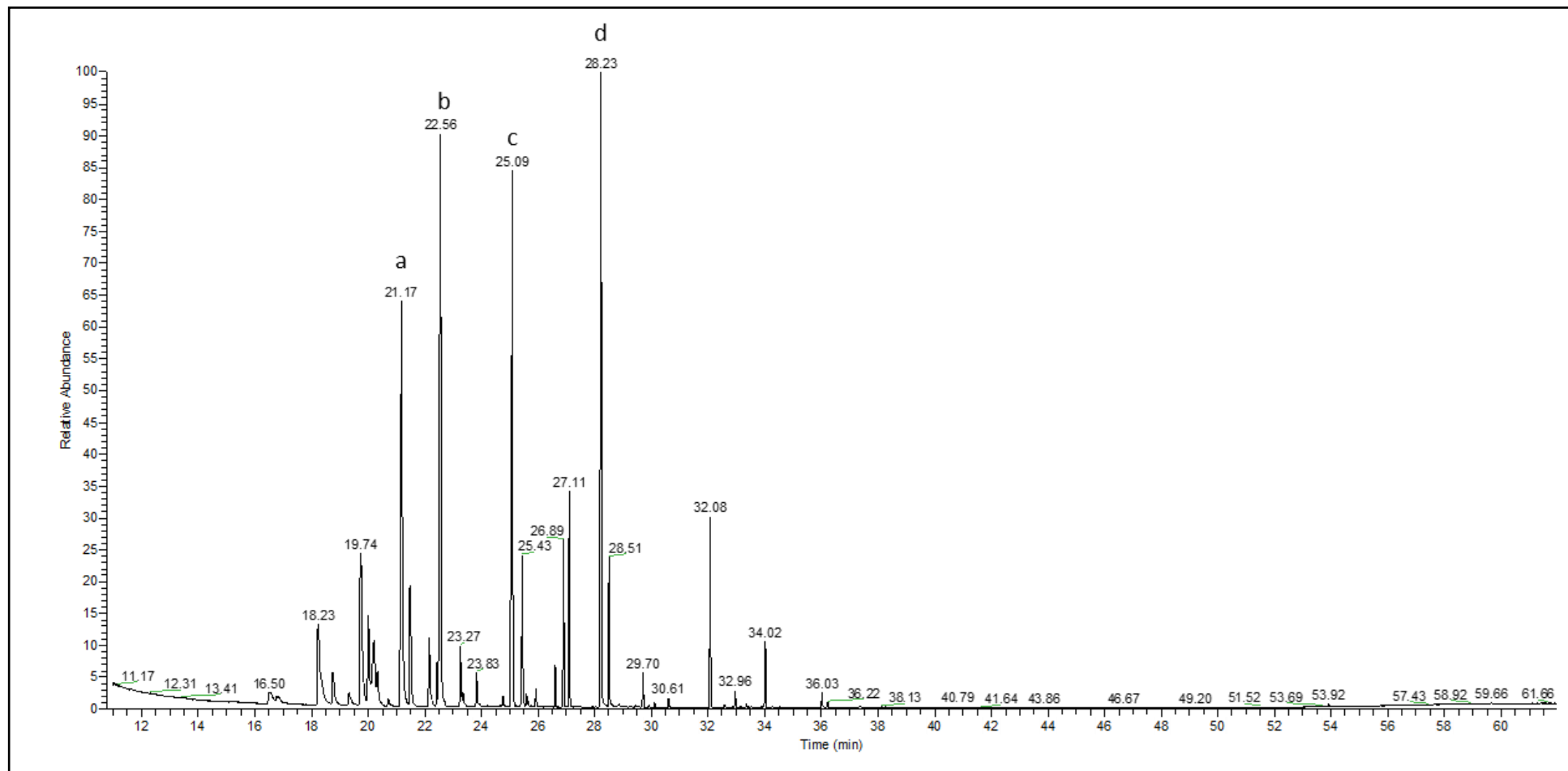
Fig. S1 GC-MS chromatogram of essential oil of O. vulgare . Letter indicate the major constituents identified in the sample. a: \gamma -terpinene; b: cis -sabinene hydrate; c: 4-terpineol; d: thymol.
