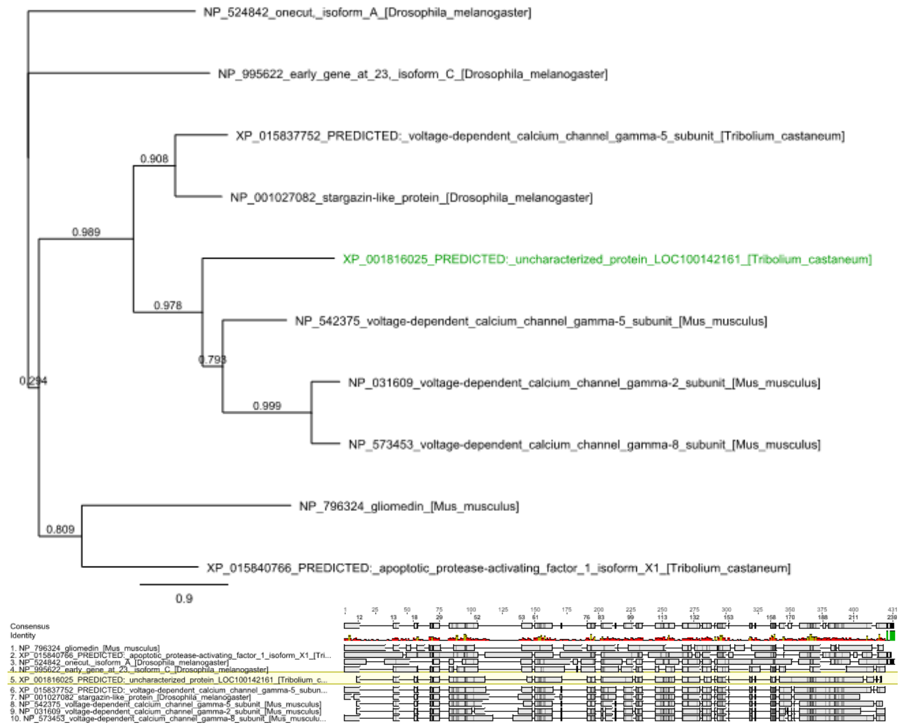
Figure S3: Phylogenetic_Tree_TC002909
