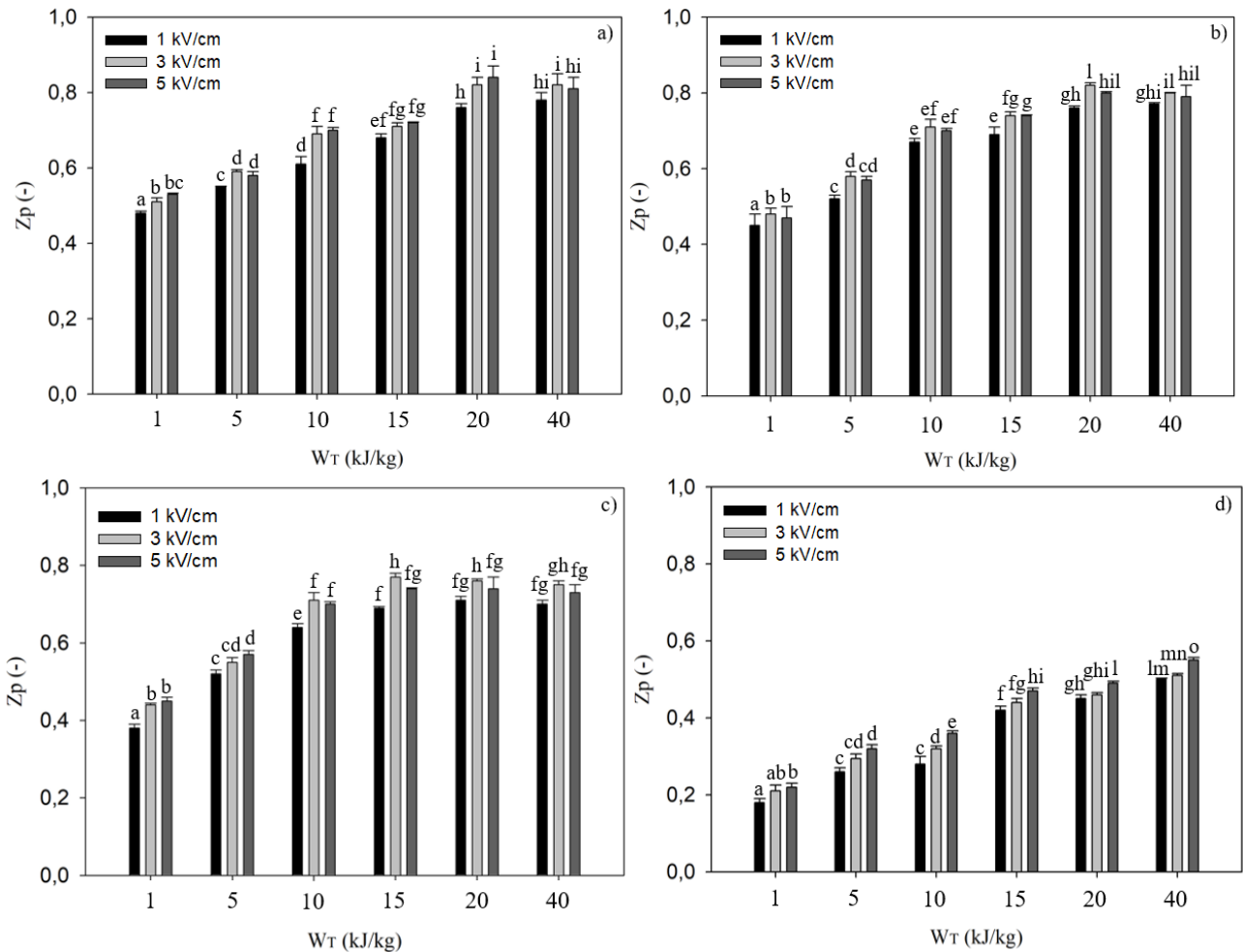
Figure S1 Cell disintegration index ( Z_p ) of vanilla pods (a), cocoa bean shells (b), vermouth mixture (c), and orange peels (d) as a function of electric field strength E (1, 3, 5 kV/cm) and total specific energy input W_T (1, 5, 10, 15, 20, 40 kJ/kg). Different letters above the bars indicate significant differences between the mean values ( p \leq 0.05 ).
