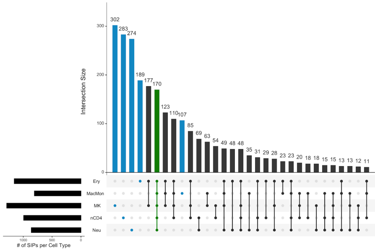
S2 Fig. A majority of SIPs are cell type-specific or shared across all five cell types. Details of SIPs are shared across cell types (black). Most SIPs, however, are cell-type specific (blue) or common between all five cell type groups (green). (Ery = erythrocytes; MacMon = macrophages/monocytes; MK = megakaryocytes; nCD4 = naive CD4 T-cells; Neu = neutrophils)
